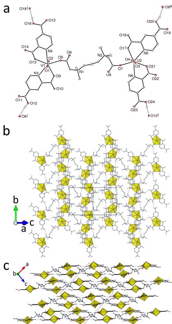
Figure 2. (a) View of compound 2 . Displacement ellipsoids are drawn at the 50% probability level. Carbon-bound hydrogen atoms are omitted and the hydrogen bonds are shown as dashed lines. Symmetry codes: i = x, y + 1, z ; j = 2 - x, y + 1/2, 3/2 - z ; k = x, y - 1, z ; l = 1 - x, y - 1/2, 1/2 - z . (b) View of one double layer of hydrogen bonded molecules. Hydrogen bonds are shown as light-blue, dotted lines. (c) Packing with double layers viewed edge-on.
