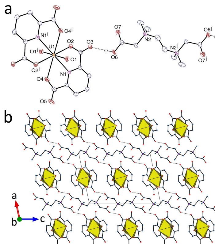
Figure 1. (a) View of compound 1. Displacement ellipsoids are drawn at the 50% probability level. Carbon-bound hydrogen atoms are omitted and the hydrogen bond is shown as a dashed line. Symmetry codes: i = 1 - x, -y, 1 - z ; j = 2 - x, 1 - y, -z . (b) View of the packing with hydrogen bonded cations and anions. Uranium coordination polyhedra are colored yellow and hydrogen bonds are shown as dotted lines.
