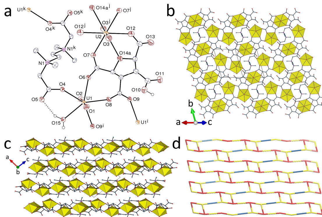
Figure 9. (a) View of compound 9 . Displacement ellipsoids are drawn at the 30% probability level. Carbon-bound hydrogen atoms are omitted and the hydrogen bond is shown as a dashed line. Only one position of the disordered atoms is represented. Symmetry codes: i = 1 - x, 1 - y, 2 - z ; j = 2 - x, -y, 1 - z ; k = 2 - x, 1 - y, 1 - z . (b) View of the fcs diperic assembly. (c) Packing with layers viewed edge-on. (d) Nodal representation of the diperic network (uranium nodes, yellow; thftcH 3- nodes, red; L1 edges, blue; view down [101] with [010] vertical).
