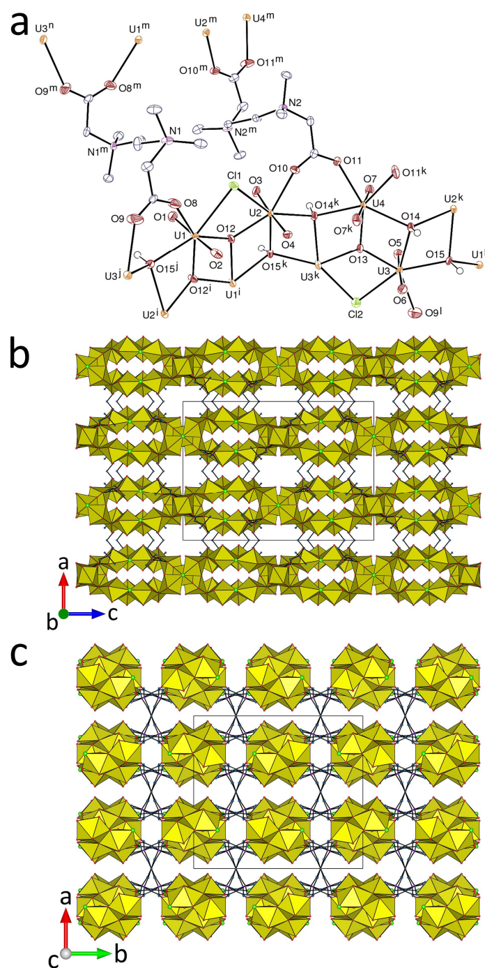
Figure 13. (a) View of compound 12. Displacement ellipsoids are drawn at the 50% probability level and carbon-bound hydrogen atoms are omitted. The disordered hydroxide close to Cl2 is not shown. Symmetry codes: i = x, 1 - y, 1/2 - z ; j = 3/2 - x, 1 - y, z - 1/2 ; k = 3/2 - x, y, 1 - z ; l = 3/2 - x, 1 - y, z + 1/2 ; m = 2 - x, 3/2 - y, z ; n = x + 1/2, y + 1/2, z - 1/2 . (b) and (c) Two views of the interpenetrated triperiodic frameworks.
