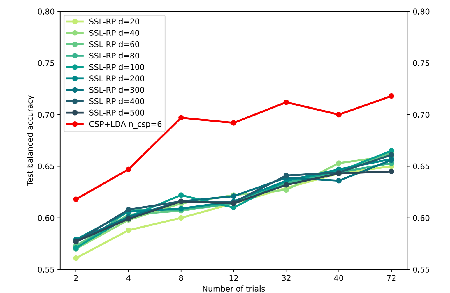
Fig. 3: Test accuracy averaged across all 9 subjects, for the detections of right or left hand MI vs rest, according to the number of training trials, obtained by the models (Self-Supervised Learning-Relative Positioning for various embedding sizes d and Common Spatial Pattern with a Linear Discriminant Analysis). The sequential training trials were randomly selected and the process was averaged for 10 repetitions.
