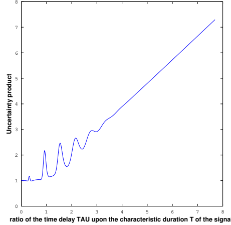
Figure 7: Uncertainty product (multiplied by 4\pi ) in term of \tau/T .
