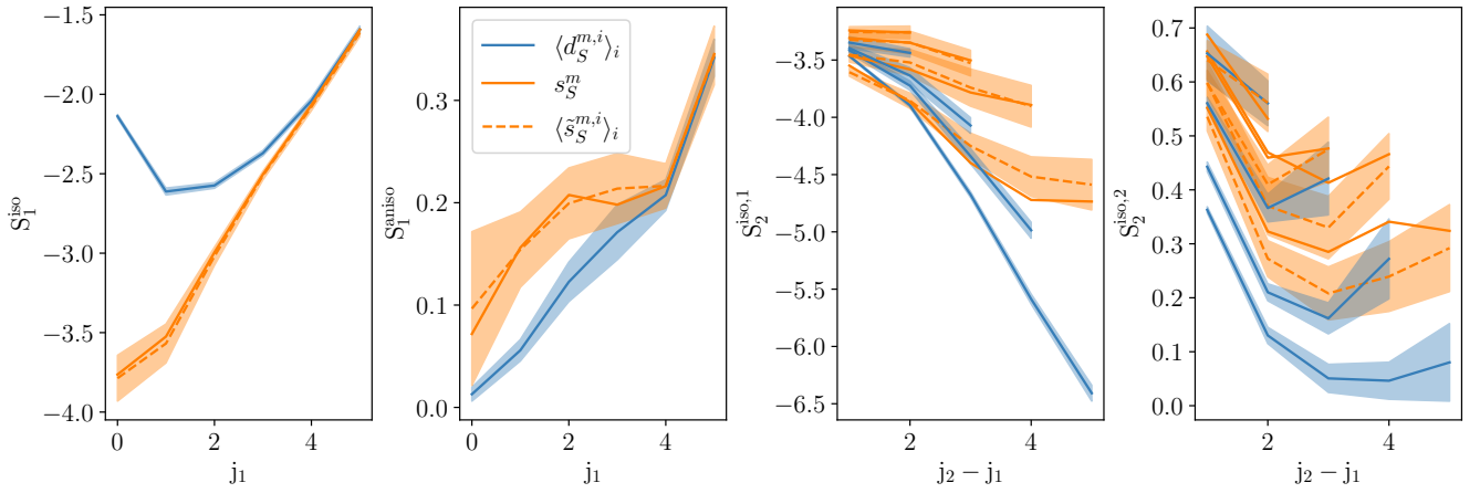
Fig. 7. RWST statistics of the input and output maps of the component separation applied to the mock data. The RWST statistics of d_S^{m,i} , s_S^m and \tilde{s}_S^{m,i} are compared. From left to right, the figure panels display S_1^{\text{iso}} (power at a given dyadic scale), S_1^{\text{aniso}} (level of anisotropy at a given dyadic scale), S_2^{\text{iso},1} (couplings between different dyadic scales), and S_2^{\text{iso},2} (angular modulation of the couplings between different dyadic scales). The variable j corresponds to the physical scale of 2^j . The S_2^{\text{iso},1} and S_2^{\text{iso},2} are normalized with respect to the S_1^{\text{iso}} and are plotted as a function of the scale ratio j_2 - j_1 for j_1 \in [0, J - 1] and j_2 \in [j_1 + 1, J - 1] . Each curve corresponds to a given j_1 . The colored bands represent the \pm 1\sigma error-bars.
