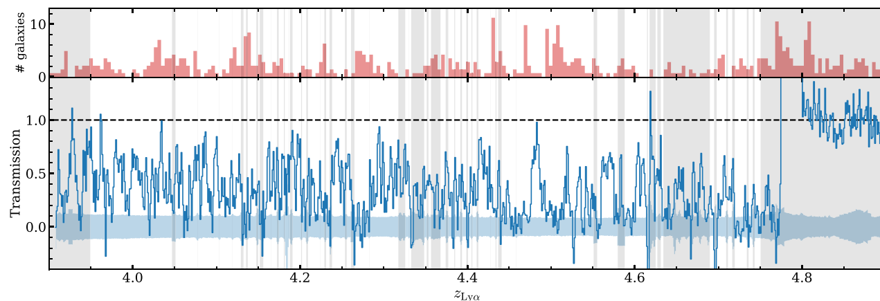
Figure 2. The H I Ly \alpha transmission in the spectrum of background galaxy ID53 at z = 4.774 (blue, bottom) compared to the foreground galaxy redshift distribution within the full field of view of MUSE surveys (red, top; the maximum impact parameter is 14 \text{ cMpc}/h_{70} ). Grey stripes highlight the regions masked due to skylines, relatively large SED model uncertainties (which are larger at metallicity-sensitive features), the locations of possible interstellar absorption lines and vicinity to ID53. Masked data were not included in measurements of the transmission or the cross-correlation between transmission and galaxy properties. The blue shaded region shows the uncertainty on the transmission, which propagates both uncertainties on the intrinsic SED of ID53 and the measurement errors of the spectrum.
