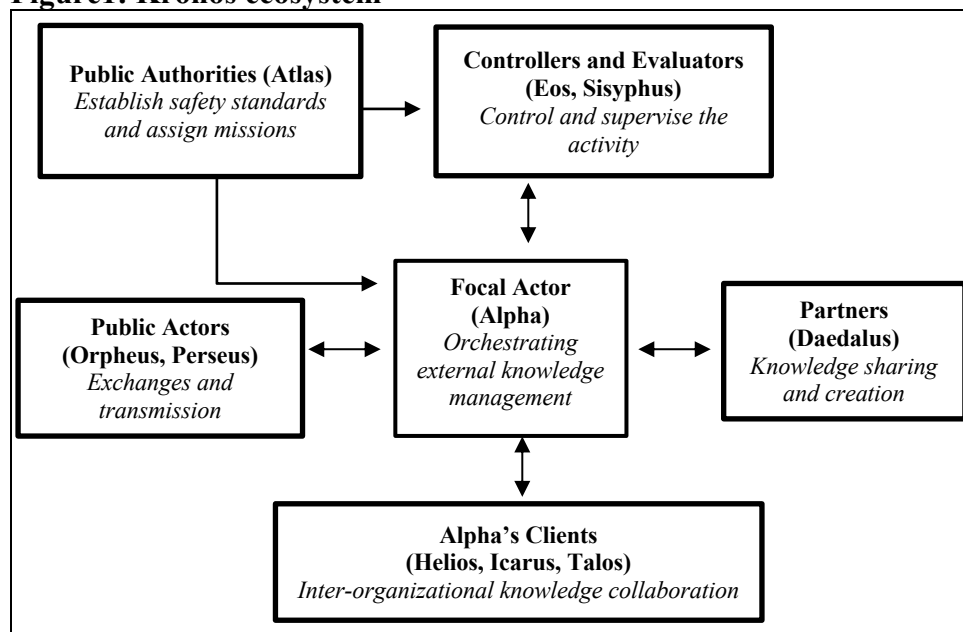
Figure1: Kronos ecosystem
