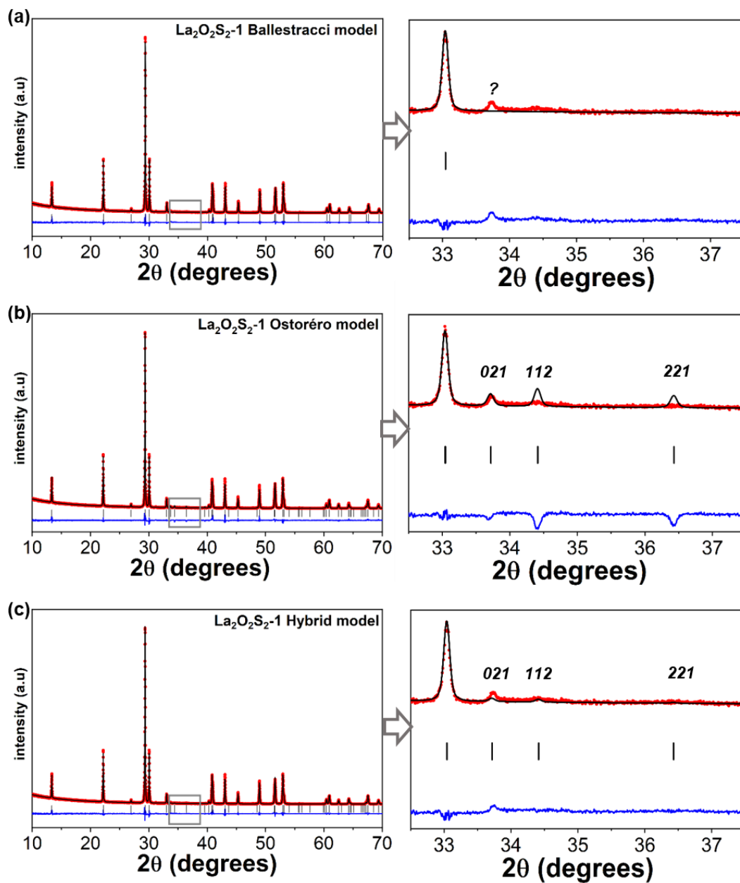
Figure 4. Rietveld refinements of \text{La}_2\text{O}_2\text{S}_2-1 with the Ballestracci model ( I4/mmm ) (a), the Ostorero model ( Cmce – one S site) (b), and the hybrid model ( Cmce – two S sites) (c). The left panels display the full diagrams while the right panels display zoom-in zooms in the 32.5-37.5 2\theta region. The black, red and blue curves represent respectively the experimental, calculated and difference diagrams. The refined Bragg positions are represented by gray vertical lines.
