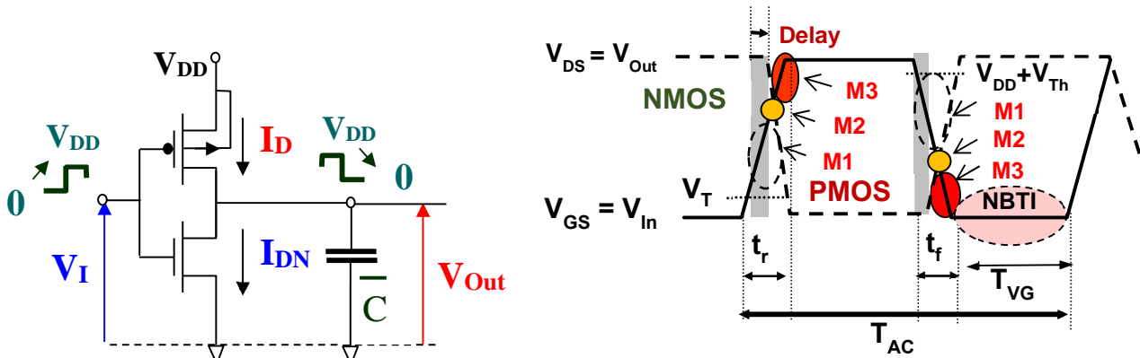
Fig. VI.19: (a) CMOS inverter operation schematics as a function of V_{In} , V_{Out} and its load capacitance CL (b) Signals applied to the inverter V_{Out} = f(V_{In}) related to the distinct bias region where HC to CC are involved (i) for NMOS transistor where V_{IN} = V_{GS,N} and V_{OUT} = V_{DS,N} while (ii) for PMOS transistor where we have V_{GS,P} = V_{IN} - V_{DD} et V_{DS,P} = V_{OUT} - V_{DD} due to the inverted potential reference for the PMOS source with V_{S,P} = V_B = V_{DD} . [111]
