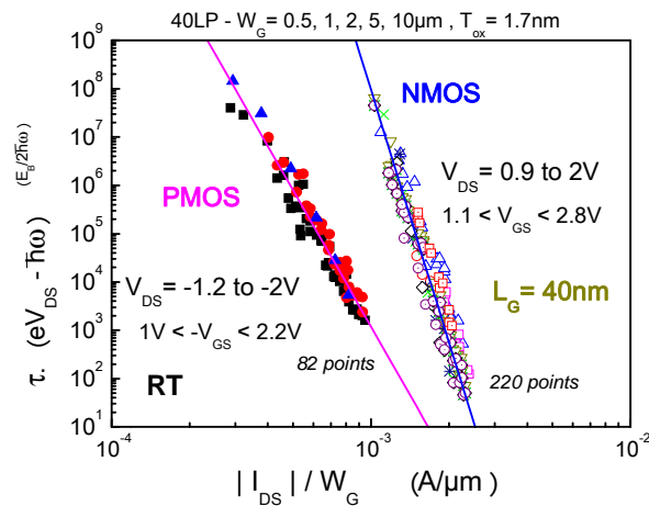
Fig. VI.6: Mode M_3 in C_{40} under CC damage according to equ. VI.6 for a large set of data in PMOS and NMOS. The M_3 degradation dependence gives a_3 = 9.4 and 17.4 , with C_3 , V_D = 7.5 \cdot 10^{-26} and 6 \cdot 10^{-45} , respectively. Same lifetime criterion 10% \Delta I_{DSat} FWD and various stressing V_{GD} that can be used for the long channel Peri COS standard from transistors in inter blocks (Fig from ref [99]).
