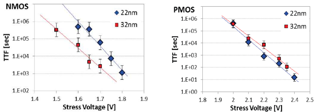
Fig.VI.5 : NMOS and PMOS TDDDB in 22nm FinFET shown as better improved with respect to 32nm that may be used for DDR3 [93]
