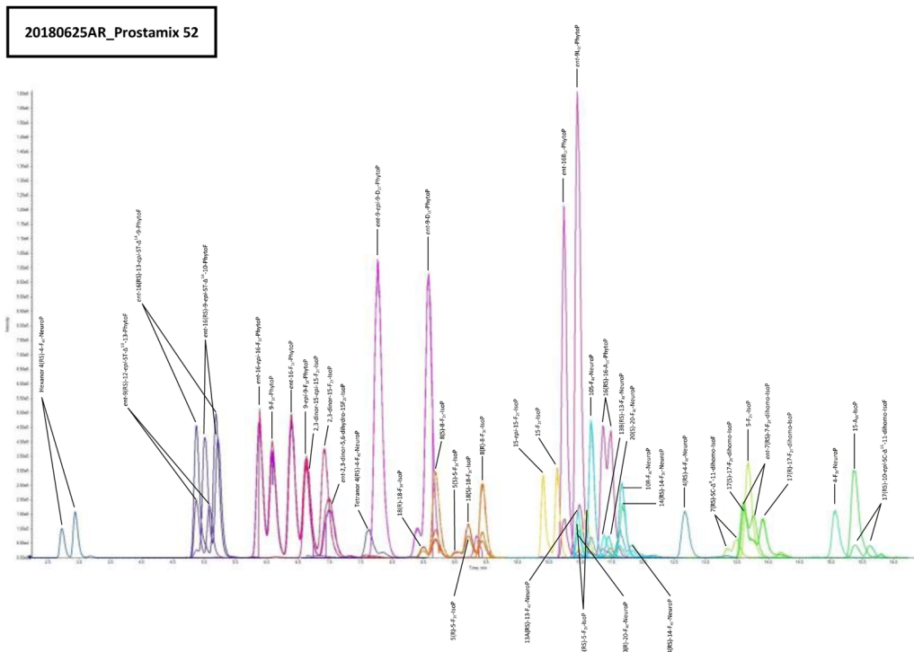
Fig. 5. LC-MS/MS > 50 isoprostanooids.
