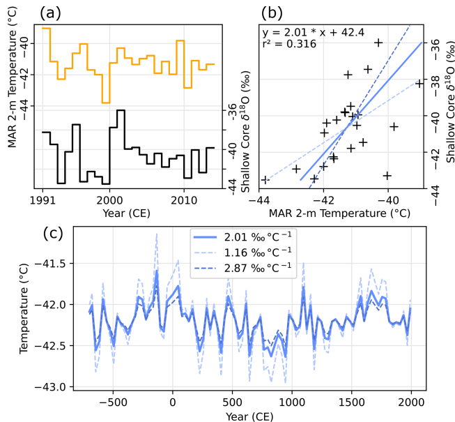
Figure 6. Calibration of the \delta^{18}\text{O} –temperature slope with the Desert Research Institute shallow core \delta^{18}\text{O} and the 2 m temperature in the Modèle Atmosphérique Régional (MAR) on the 1991–2013 CE period. (a) Annually averaged series of MAR 2 m temperature (orange) and shallow core \delta^{18}\text{O} on the 1991–2013 period. (b) Scatter plot of the two datasets (black crosses), with linear regression shown as a blue solid line. Dashed lines represent the slope upper and lower uncertainties at a 95 % confidence level. (c) Temperature reconstruction using the \delta^{18}\text{O} series from the ABN1314 core and the slope obtained with linear regression, with temperature reconstructed with upper and lower uncertainty slope values shown as dashed lines.
