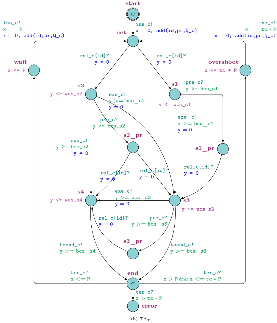
Figure 3: TA_\tau (Fig 2) and \mathcal{H}_c with synchronizations. Notice the committed locations in \mathcal{H}_c to enforce sequences of timeless actions corresponding to scheduling decisions. For instance, location insert is committed to force inserting all tasks activated at the same time one after another without interference from other actions, thus removing unnecessary interleaving.
