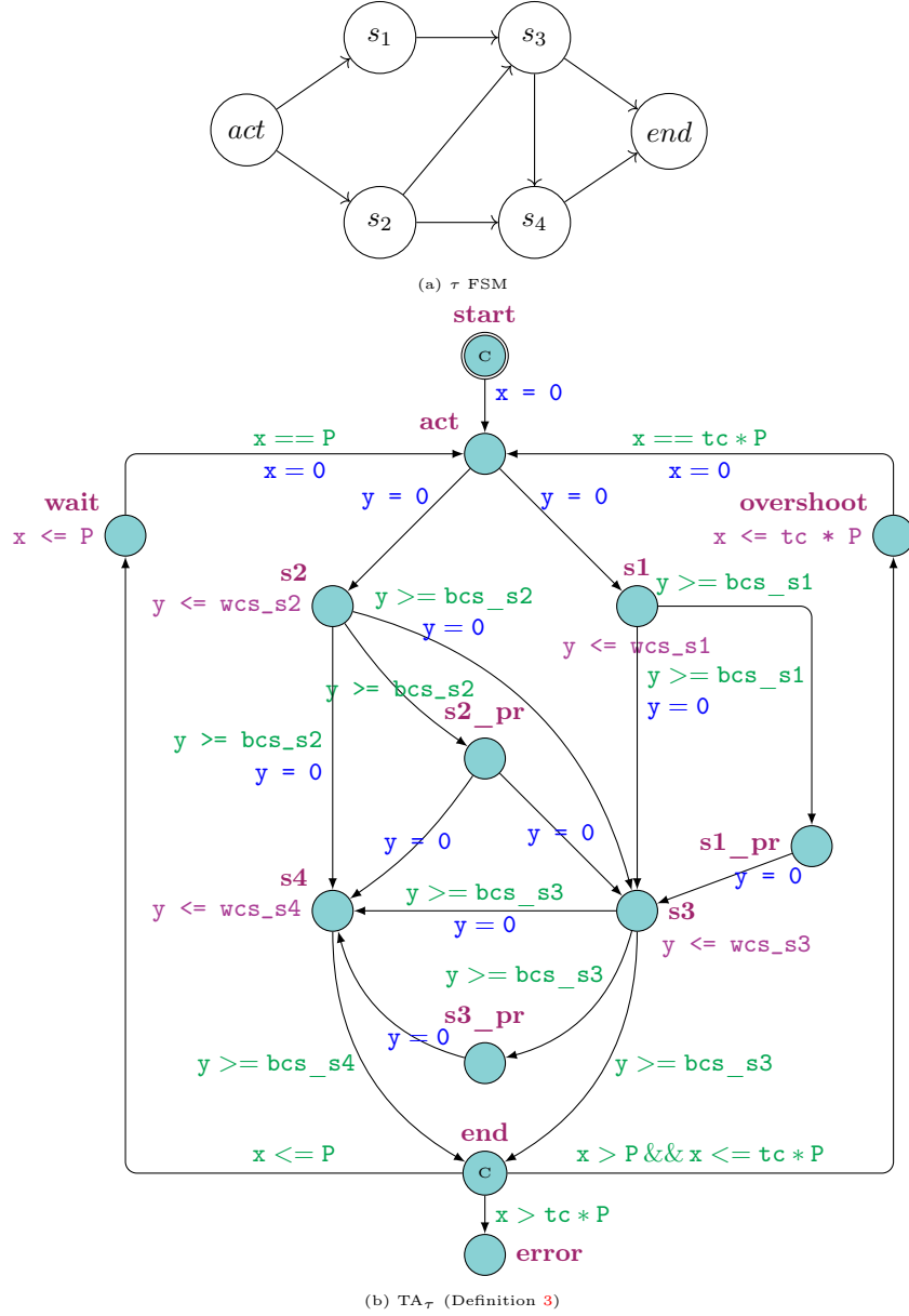
Figure 2: FSM and resulting TA model (in UPPAAL notation) for a task \tau . P is a constant equal to p(\tau) . Note that x = 0 on edge start \rightarrow act is superfluous since start is both committed and initial (this edge is taken at x = 0 anyways, see the synchronized model in Fig. 3). Note also that tc is upperbounded by 2, i.e., this representation is valid for tc = 1 (in which case location overshoot is superfluous) or tc = 2 , and therefore variable na is not needed and there is only one edge from end to overshoot .
