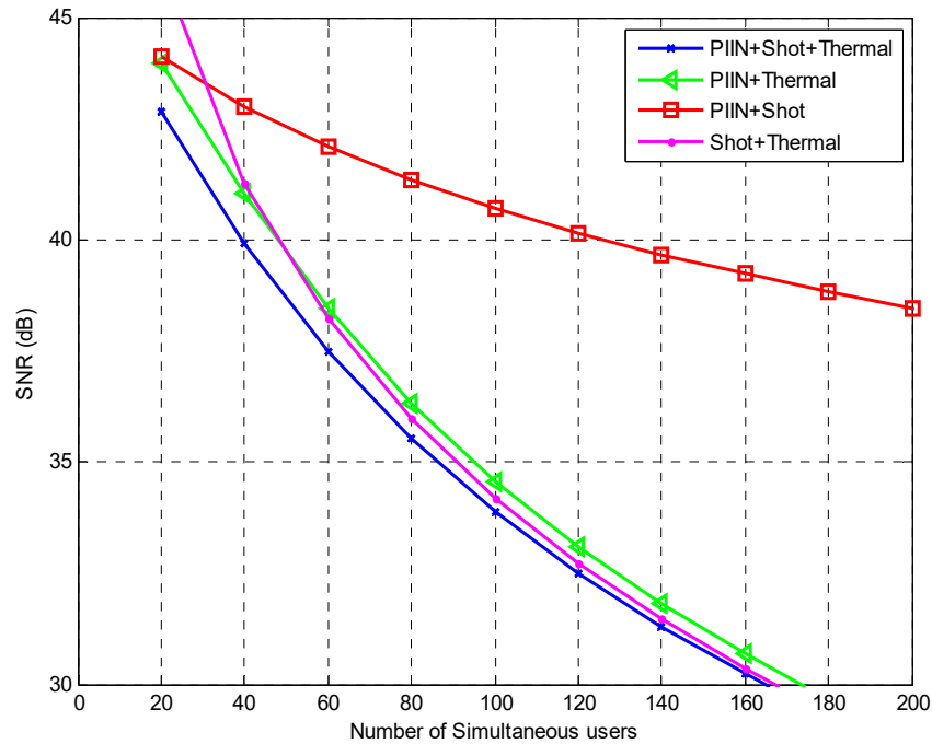
Figure 9. SNR versus number of simultaneous users for different noise sources.
