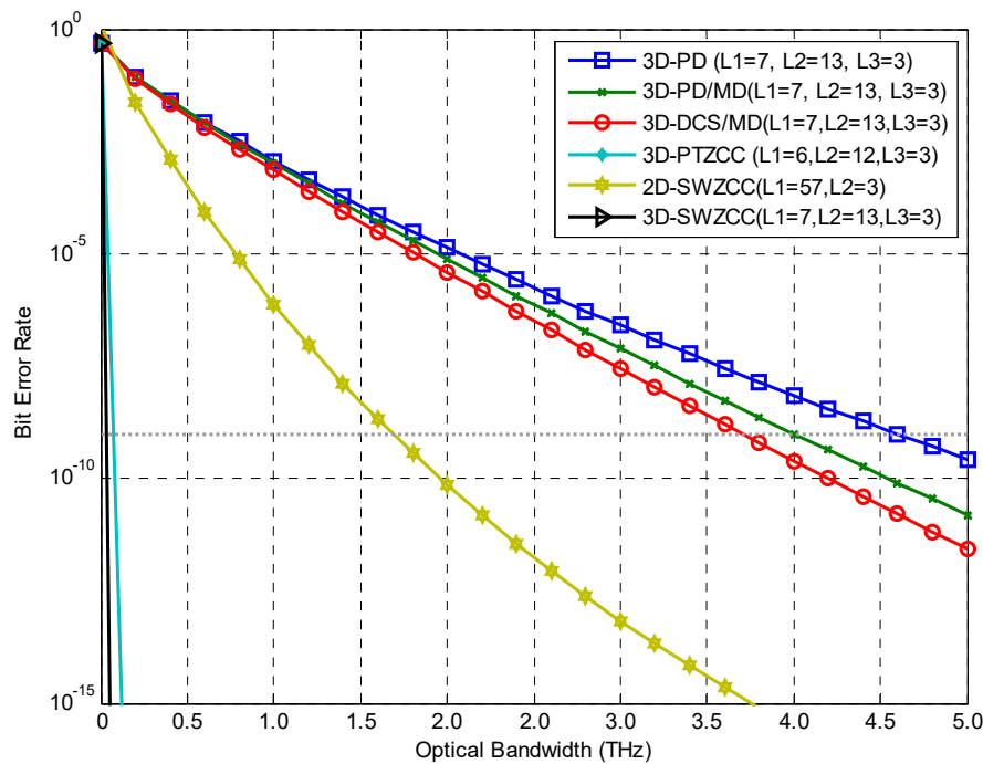
Figure 8. BER versus optical bandwidth for K = 100.
