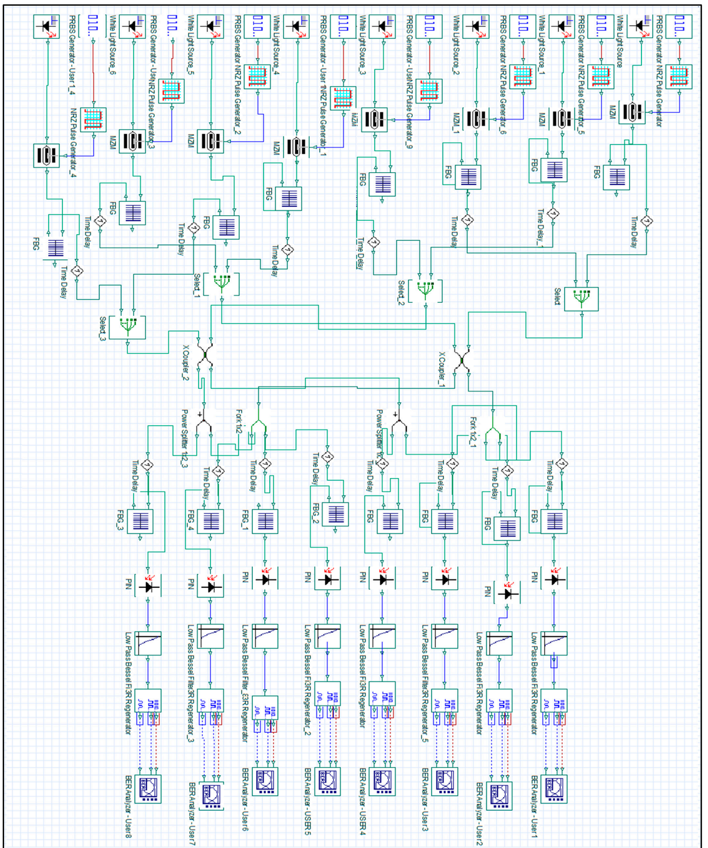
Figure 15. Block diagram of the 3D-OCDMA system.
