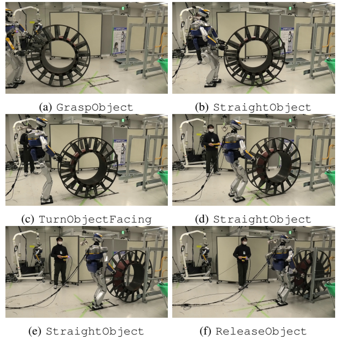
Fig. 11: Motion actions for the HRP-2KAI bobbin experiment.
