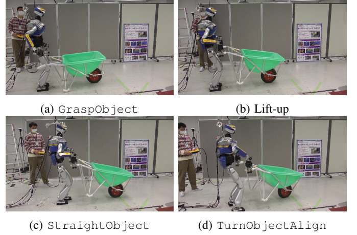
Fig. 10: HRP-2KAI's experiment moving the wheelbarrow.
