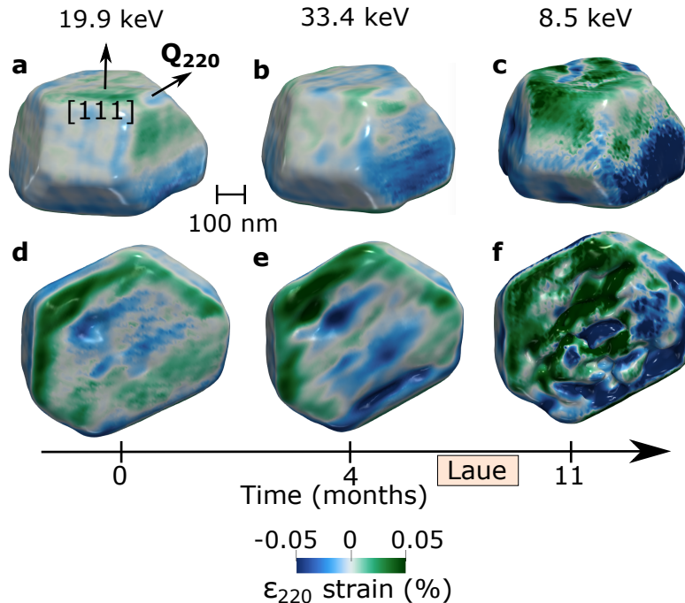
Figure 4: \epsilon_{220} strain . Evolution of the strain along the [220] direction of the Pt particle recovered from Bragg coherent diffraction imaging measurements at 19.9 keV (a, d), 33.4 keV (b, e) and 8.5 keV (c, f). The top (bottom) row shows a side (bottom) three-dimensional view of the particle. The reconstructed electron density of the Pt particle is drawn at 30% (50%) at 8.5 keV (at 19.9 keV and 33.4 keV) of the maximum electron density. The isosurface value of the electron density (coloured with the retrieved \epsilon_{220} strain) has been chosen based on the criterion described in Ref. 32 The chronology of the measurements is displayed on the x axis, highlighting when Laue measurements were made.
