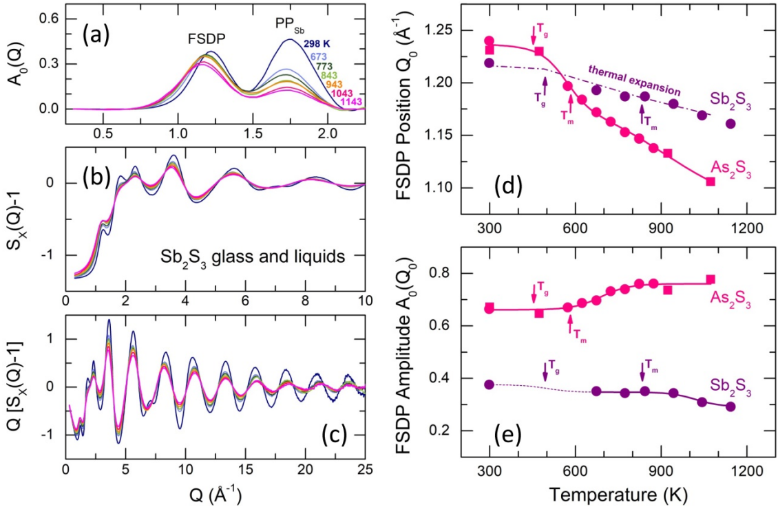
Figure 6. High-energy X-ray diffraction data in Q -space for glassy and liquid Sb 2 S 3 : (a) isolated first sharp diffraction peak (FSDP) and Sb-Sb diffraction feature PP Sb as a function of temperature; (b) X-ray structure factor S_X(Q) over a limited Q -range and (c) interference function Q[S_X(Q)-1] as a function of temperature; (d) the FSDP position Q_0(T) and (e) amplitude A_0(Q_0, T) for antimony and arsenic sesquisulfides. The dash-dotted line for Sb 2 S 3 in (d) shows the expected Q_0(T) trend taking into account the thermal expansion. The arrows show the glass transition temperature T_g and melting point T_m for As 2 S 3 and Sb 2 S 3 . The solid and dashed lines in (d) and (e) are a guide to the eye.
