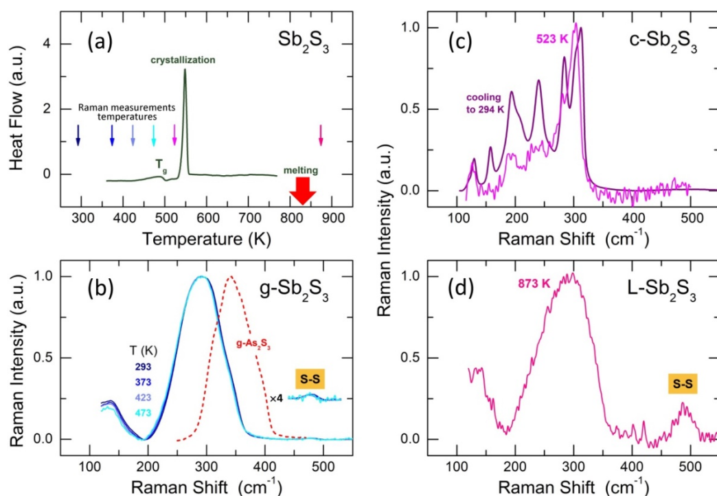
Figure 4. Raman spectra of antimony sesquisulfide: (a) DSC trace of g - \text{Sb}_2\text{S}_3 , the arrows show the Raman measurement temperatures; (b) spectra of a solid glass as a function of temperature, the insert shows S-S stretching at \approx 490 \text{ cm}^{-1} ; (c) spectra of orthorhombic polymorph at 523 K and after cooling to room temperature; (d) Raman spectrum of molten \text{Sb}_2\text{S}_3 at 873 K. The dashed red line in (b) also shows the As-S stretching envelope in g - \text{As}_2\text{S}_3 . See text for further details.
