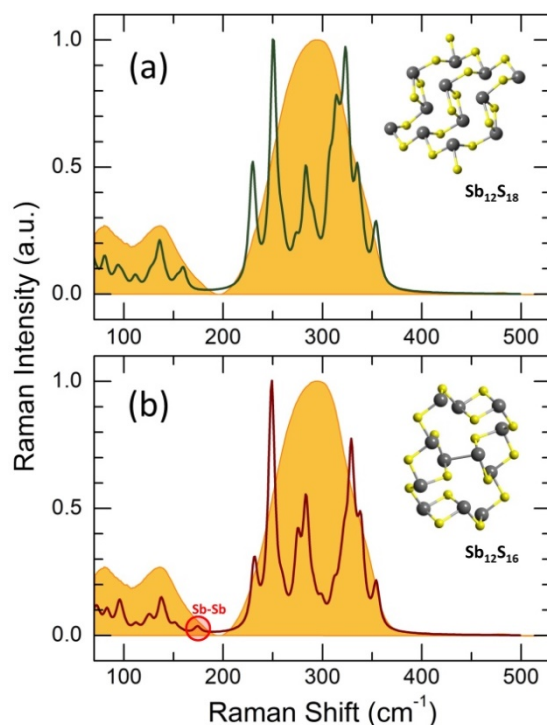
Figure 5. DFT Raman spectra of (a) \text{Sb}_{12}\text{S}_{18}\text{H}_2 and (b) \text{Sb}_{12}\text{S}_{16} size-limited clusters in comparison with experimental Raman spectrum of g - \text{Sb}_2\text{S}_3 , highlighted in yellow for the two panels. The terminal hydrogen species in (a) are omitted, and the H-related vibrations are removed from the spectrum. The inserts show DFT-optimized clusters. Weak Sb-Sb stretching in (b) is emphasized by the red circle.
