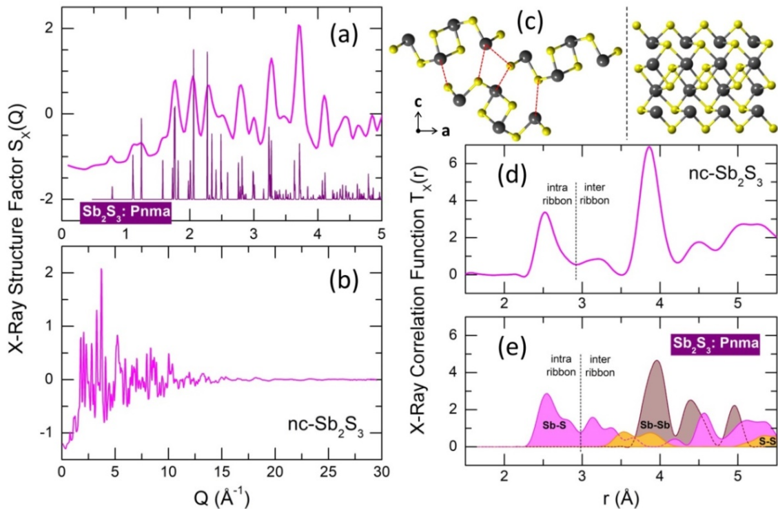
Figure 3. Nanocrystalline ( nc ) and orthorhombic \text{Sb}_2\text{S}_3 . (a) Bragg peaks of the nanocrystalline sample in comparison with orthorhombic polymorph 16 , space group Pnma ; (b) X-ray structure factor S_X(Q) over the entire Q -range; (c) (\text{Sb}_4\text{S}_6)_\infty ribbons in orthorhombic \text{Sb}_2\text{S}_3 : left , atomic arrangements using projection on the (a, c) plane, right , a single ribbon oriented parallel to the b axis; (d) X-ray total correlation function T_X(r) of nc\text{-Sb}_2\text{S}_3 ; (e) \text{Sb-S} (magenta), \text{Sb-Sb} (light brown) and \text{S-S} (yellow) T_{ij}(r) partials for orthorhombic \text{Sb}_2\text{S}_3 . The dashed red lines in (c), left panel, show the shortest inter-ribbon \text{Sb-S} distances (3.167-3.642 \text{\AA} ). The black dashed lines in (d) and (e) separate intra- (2.455-2.854 \text{\AA} ) and inter-ribbon \text{Sb-S} nearest contacts.
