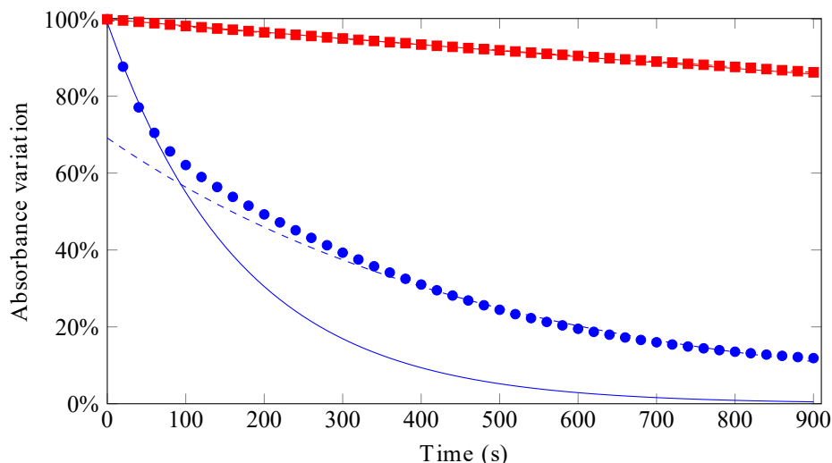
Figure 5: Normalized bleaching of the solution containing pNDA ( 90 \mu\text{M} ), MB ( 20 \mu\text{M} ) in PBS ( \text{pH} = 7.4 ) with \bullet or without \blacksquare L-histidine ( 5 \text{ mM} ) irradiated with red LEDs for 15 min. The different experiments data are shown by the geometrical shapes and their modeling is represented by the continuous line for initial rate and by the dashed line for established rate. All models are statistically significant ( p < 4 \times 10^{-3} ).
