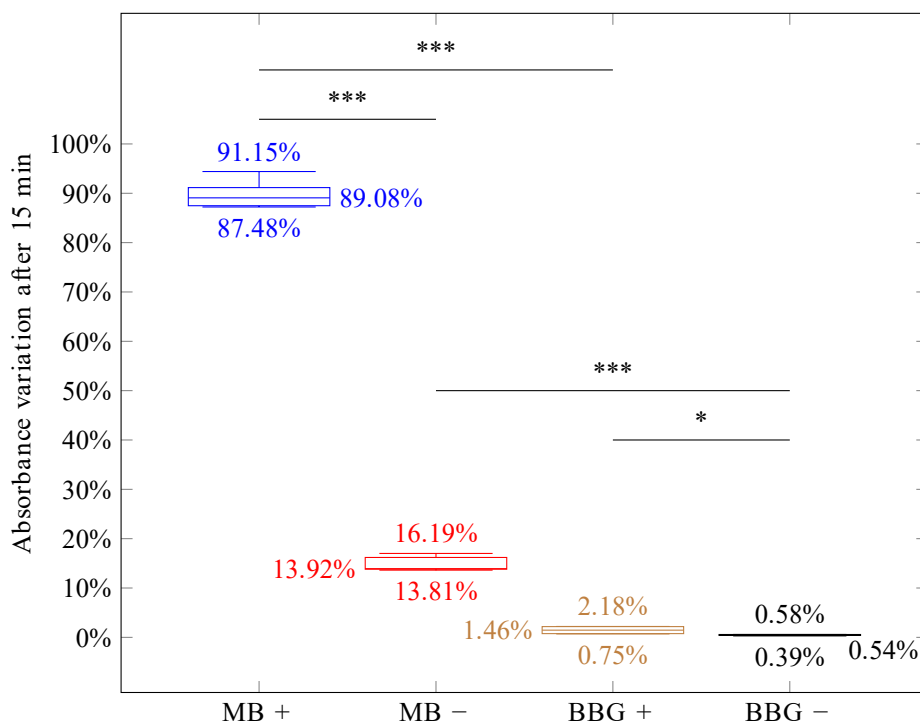
Figure 9: Normalized bleaching of the solution containing pNDA (90 \mu\text{M} ) and MB (20 \mu\text{M} ) ● ● or BBG (20 \mu\text{M} ) ● ● in PBS (pH = 7.4) with (+) ● ● or without (-) ● ● L-histidine (5 mM) after a red LEDs 15-minute irradiation. Each box is the average six experimental data. The numerical values shown are, from top to bottom, the upper quartile, the median and the lower quartile. All model are statistically significant ( p < 0.001 ) and *** is for p \leq 0.001 and * for p \leq 0.05 .
