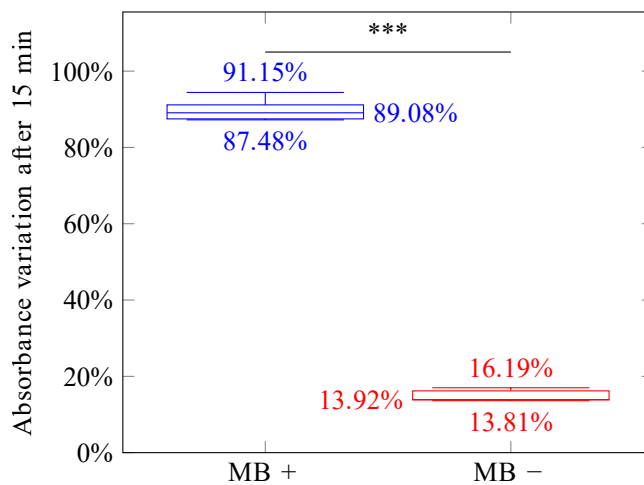
Figure 6: Normalized bleaching of the solution containing pNDA ( 90 \mu\text{M} ), PBS ( \text{pH} = 7.4 ) and MB ( 20 \mu\text{M} ) with (+) \bullet or without (-) \bullet L-histidine ( 5 \text{ mM} ) after a red LEDs 15-minute irradiation. Each box is the average six experimental data. The numerical values shown are, from top to bottom, the upper quartile, the median and the lower quartile. All models are statistically significant ( p < 0.01 ) and *** is for p \leq 0.001 .
