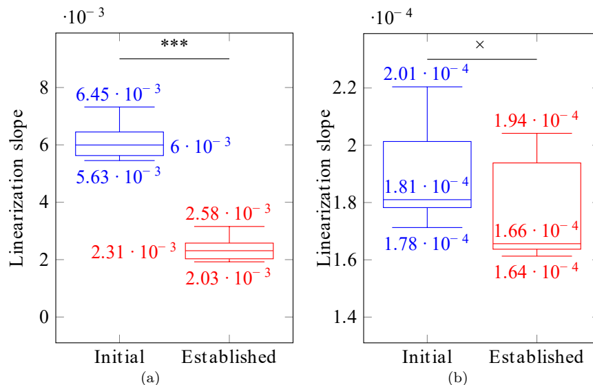
Figure 7: Linearization slopes of the bleaching of solutions containing pNDA ( 90 \mu\text{M} ) and MB ( 40 \mu\text{M} ) in PBS ( \text{pH} = 7.4 ) with (a) or without (b) L-histidine ( 5 \text{ mM} ) irradiated with red LEDs for 15 min. Each data set is modeled with two limit cases of initial \bullet and established rate \bullet . Each box is the average six experimental data. The numerical values shown are, from top to bottom, the upper quartile, the median and the lower quartile. All models are statistically significant ( p < 0.001 ) and \times is for p > 0.1 and *** for p \leq 0.001 .
