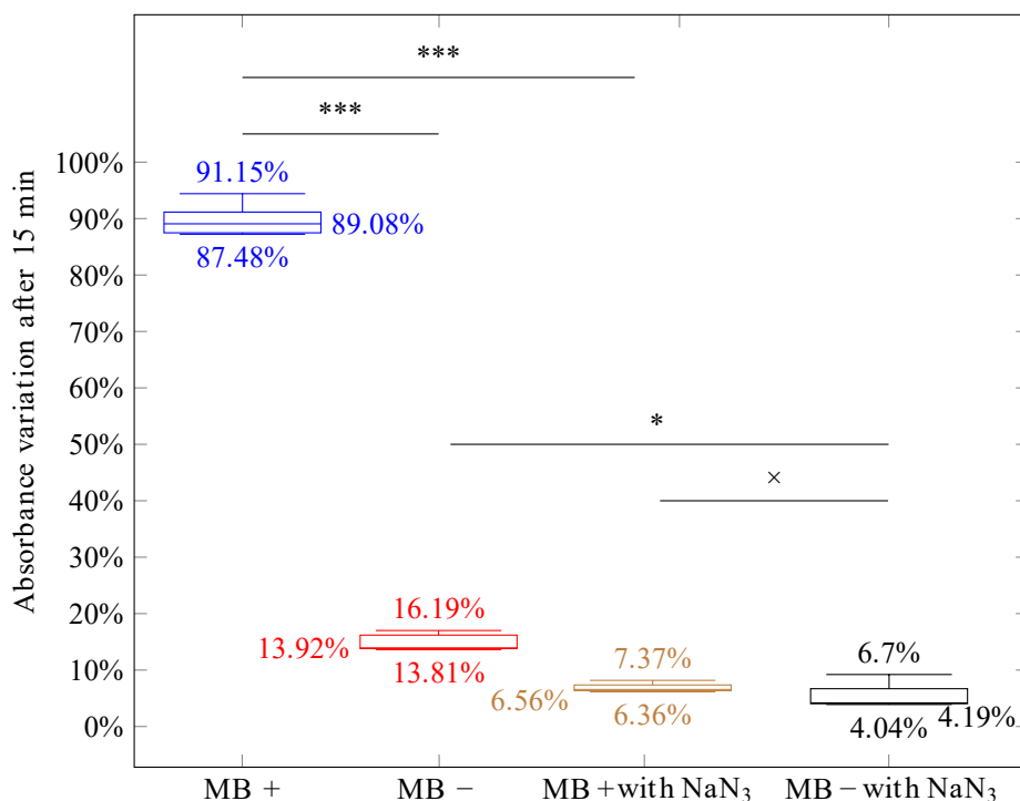
Figure 8: Normalized bleaching of the solution containing pNDA ( 90 \mu\text{M} ) and MB ( 20 \mu\text{M} ) in PBS ( \text{pH} = 7.4 ) with (+) ● or without (-) ● L-histidine ( 5 \text{ mM} ) and with ● or without ● sodium azide ( 5 \text{ mM} ) after a red LEDs 15-minute irradiation. Each box is the average six experimental data without scavenger and three experimental data with scavenger. The numerical values shown are, from top to bottom, the upper quartile, the median and the lower quartile. All models are statistically significant ( p < 0.001 ) and *** is for p \leq 0.001 , * for p \leq 0.05 and \times for p > 0.1 .
