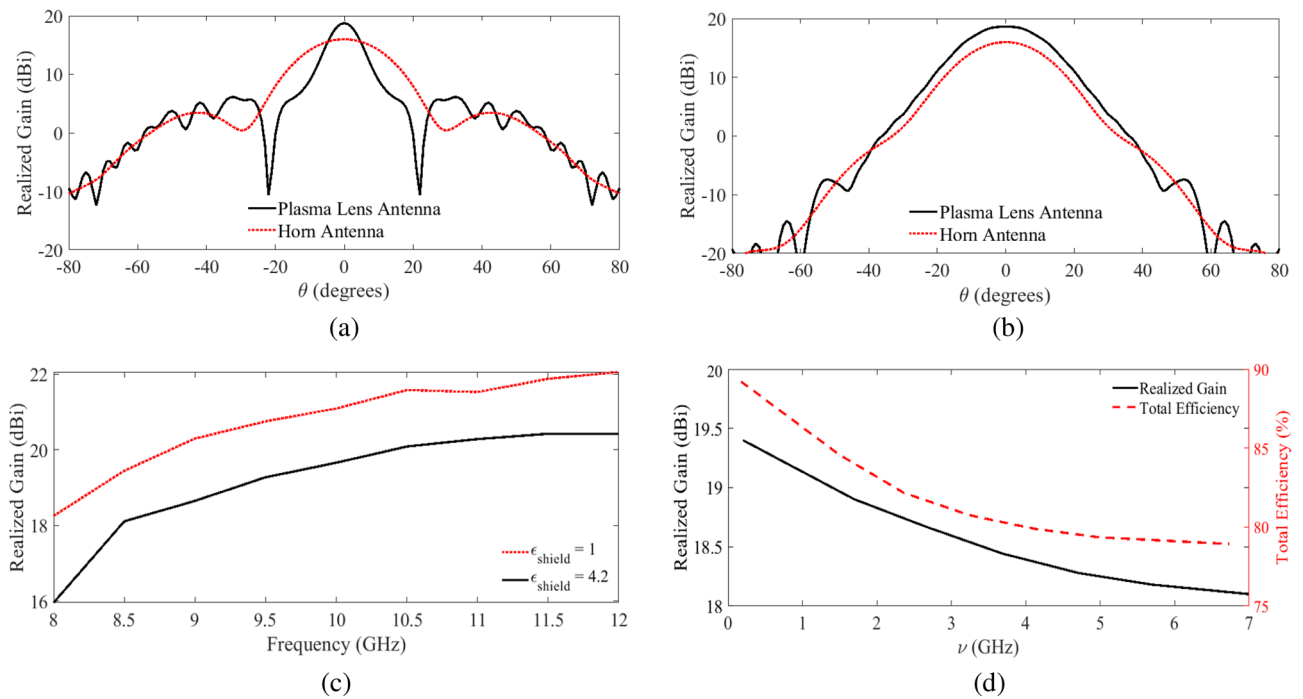
Figure 7. (a) A comparison between the radiation gain in the E-plane of the one-dimensional biconcave plasma lens antenna and the standard horn feed at 10 GHz, (b) a comparison between the radiation gain in the H-plane, (c) simulated realized gain versus the frequency for the plasma lens antenna with \epsilon_{shield} = 4.2 and \epsilon_{shield} = 1 , and (d) simulated realized gain and total efficiency of the lens antenna versus the collision frequency of the plasma.
