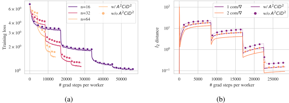
Figure 5: (a) Training loss for ImageNet using 128 batch size, with an equal number of communications and computations per worker. We display the training loss for various number of workers (up to 64), using \mathbf{A}^2\mathbf{CiD}^2 , for the ring graph. (b) Comparison of consensus distances when \mathbf{A}^2\mathbf{CiD}^2 is applied versus doubling the rate of communications on the ring graph with 64 workers: applying \mathbf{A}^2\mathbf{CiD}^2 has the same effect as doubling communications.
