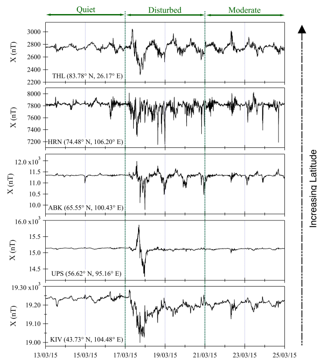
Figure 3. The X component of the geomagnetic field measured at five different observatories between 13 and 24 March 2015, located at different magnetic latitudes (increasing from bottom to top). The green dotted lines demarcate time intervals distinguished by different levels of geomagnetic activity.
