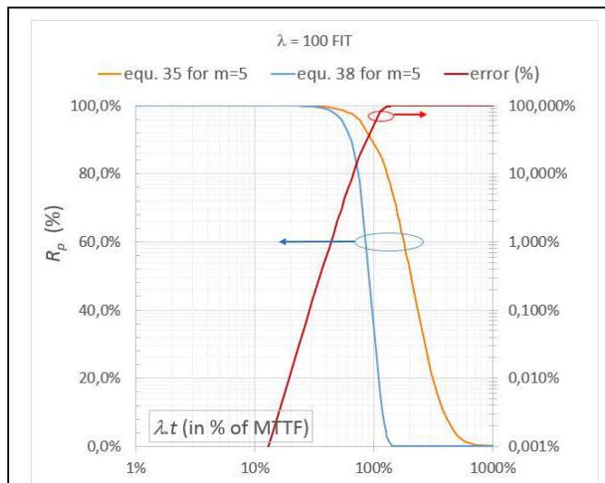
Figure V-11: Plot error (in red) as the difference between plot of Eq. 35 and Eq.38 for a POISSON Distribution with \lambda=100 FIT, \beta=m=5 .
