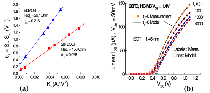
Fig.3: (a) Direct extraction of \theta_{10} (Y-intercept) and R_{SDo} (slope) that is compared to the product of Y = I_{DS}/G_m^{0.5} and X = G_m^{-0.5} functions [22] in fresh 28FD and EDMOS devices. (b) Corresponding linear I_{DS} - V_{GS} dependence in 28FD compared between models (lines) and measurements (labels) under HCD M3 mode ( V_{GS} > V_{DS} ).
