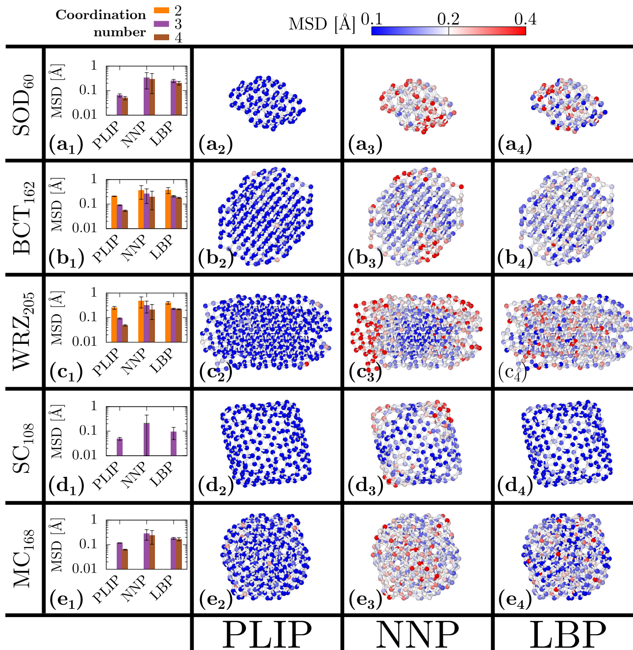
FIG. 7. Influence of the coordination number on the MSD error for five typical nanoparticles and for each considered models. Coordination numbers are computed with a cutoff equal to 2.5 \text{ \AA} .
