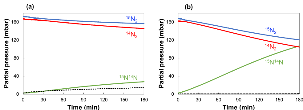
Fig. 5. Nitrogen isotopic distribution during ^{15}\text{N}_2/^{14}\text{N}_2 homomolecular exchange at 500 °C over (a) Ru/LaScSiH 1.5 and (b) Ru/LaScSiH 1.5 partially dehydrogenated (hereafter denoted as Ru/LaScSiH x ) after 2 h treatment under Ar flow at 500 °C (dashed line represents the evolution of the partial pressure of H 2 from signal m/z = 2 ).
