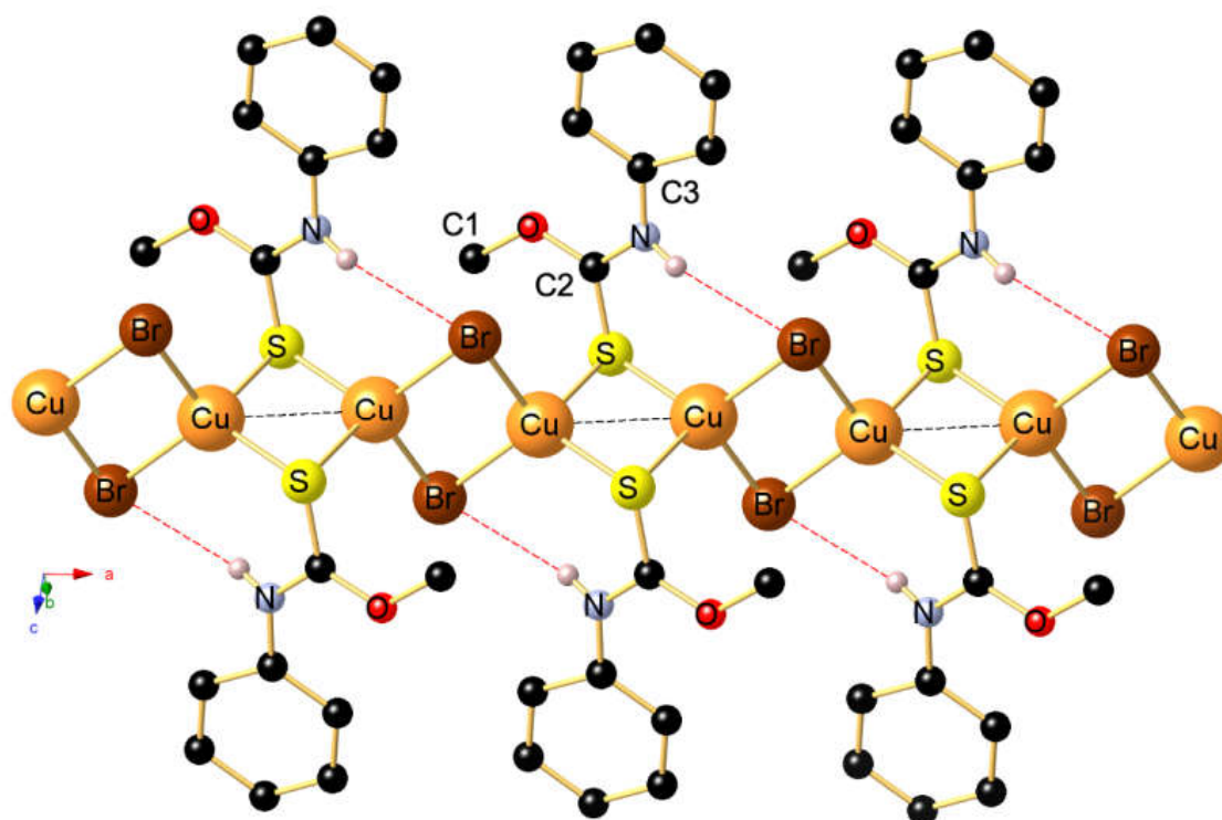
Figure 1. Crystal structure of the 1D ribbon of [\text{Cu}(\mu_2\text{-Br})_2\text{Cu}](\mu_2\text{-L})_2 CP1 running along the a axis. Selected bond lengths (Å) and angles (deg) of CP1: \text{Cu}\cdots\text{Cu}^1 2.8649(10), \text{Cu}\text{-Cu}^2 2.8339(10), \text{Br}\text{-Cu} 2.4620(7), \text{Cu}\text{-S} 2.2966(12), \text{Cu}\text{-S}^2 2.4157(12), \text{S}\text{-C}1 1.711(5), \text{O}\text{-C}1 1.313(5), \text{O}\text{-C}2 1.453(5), \text{N}\text{-C}1 1.335(5), \text{N}\text{-C}3 1.421(6); \text{Cu}^2\text{-Cu}\text{-Cu}^1 171.28(5), \text{S}\text{-Cu}\text{-Br} 117.68(4), \text{S}\text{-Cu}\text{-Br}^1 107.64(4), \text{S}\text{-Cu}\text{-S} 106.11(4), \text{Br}\text{-Cu}\text{-Br}^1 109.12(2), \text{Br}\text{-Cu}\text{-Cu}^1 54.83(2), \text{Br}\text{-Cu}\text{-Cu}^2 130.17(3), \text{Br}^1\text{-Cu}\text{-Cu}^2 120.12(3), \text{S}\text{-Cu}\text{-Cu}^1 131.40(4), \text{S}\text{-Cu}\text{-Cu}^2 51.13(3), \text{S}\text{-Cu}\text{-Cu}^1 131.30(4), \text{N}\text{-C}1\text{-S} 121.7(3), \text{C}8\text{-C}3\text{-N} 115.3(4), and \text{C}7\text{-C}8\text{-C}3 120.4(3). Symmetry transformation used to generate equivalent atoms: 1 2-x, 1-y, 2-z ; 2 1-x, 1-y, 2-z .
