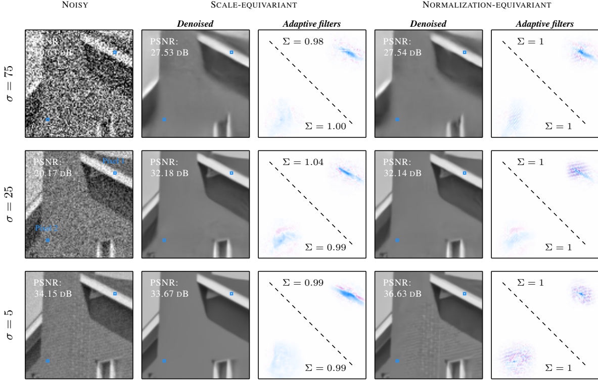
Figure 6: Visual comparisons of the generalization capabilities of a scale-equivariant FDCNN [30] (left) and its normalization-equivariant counterpart (right) for Gaussian noise. Both networks were trained for Gaussian noise at noise level \sigma = 25 exclusively. The adaptive filters (rows of A_{\theta}^{y_r} in Prop. 4) are indicated for two particular pixels as well as the sum of their coefficients (note that some weights are negative, indicated in red). The scale-equivariant network tends to excessively smooth out the image when evaluated at a lower noise level, whereas the normalization-equivariant network is more adaptable and considers the underlying texture to a greater extent.
