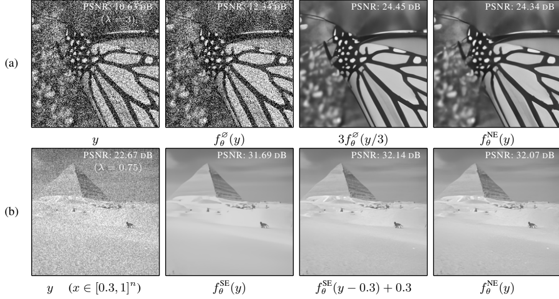
Figure 8: Denoising results for example images of the form y = x + \lambda \varepsilon with \sigma = 25/255 and x \in [0, 1]^n , by FDnCNN [30] specialized for noise level \sigma only. Here, f_{\theta}^O , f_{\theta}^{SE} and f_{\theta}^{NE} denote the ordinary , scale-equivariant and normalization-equivariant variants, respectively.
