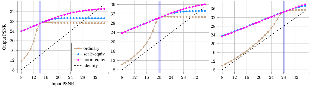
Figure 7: Comparison of the performance of our normalization-equivariant FDCNN [30] with its scale-equivariant and ordinary counterparts for Gaussian denoising on the Set12 dataset. The vertical blue line indicates the unique noise level on which the networks were trained exclusively (from left to right: \sigma = 50 , \sigma = 25 and \sigma = 10 ). In all cases, normalization-equivariant networks generalize much more robustly beyond the training noise level.
