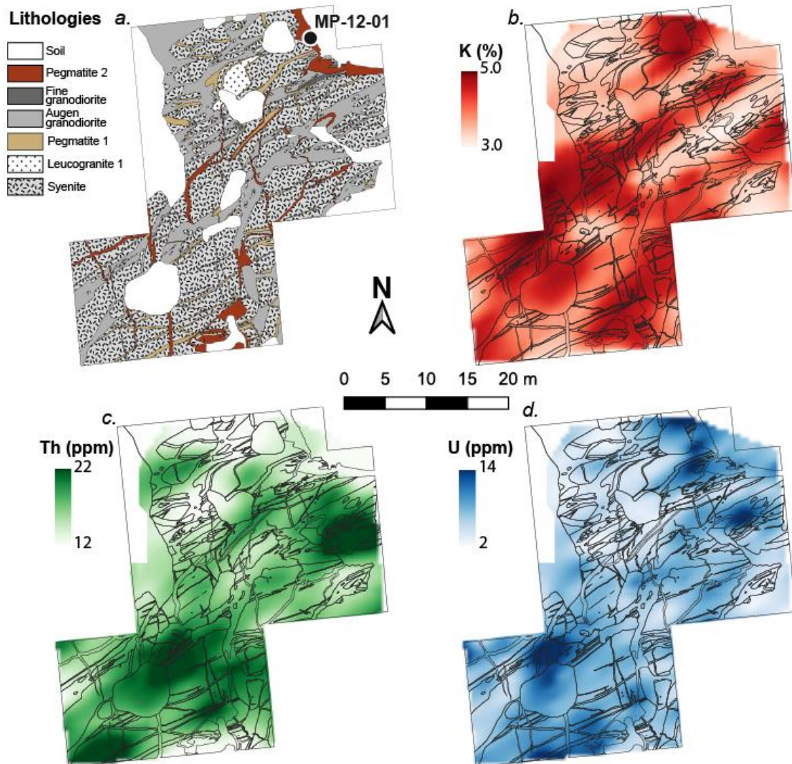
Figure 10. Lithological (a) and gamma-ray (b—d) maps for the “Eagle High” outcrop. Only the interpolated grids are shown for each element. The location of sample MP-12-01, studied for autoradiography, is indicated.
