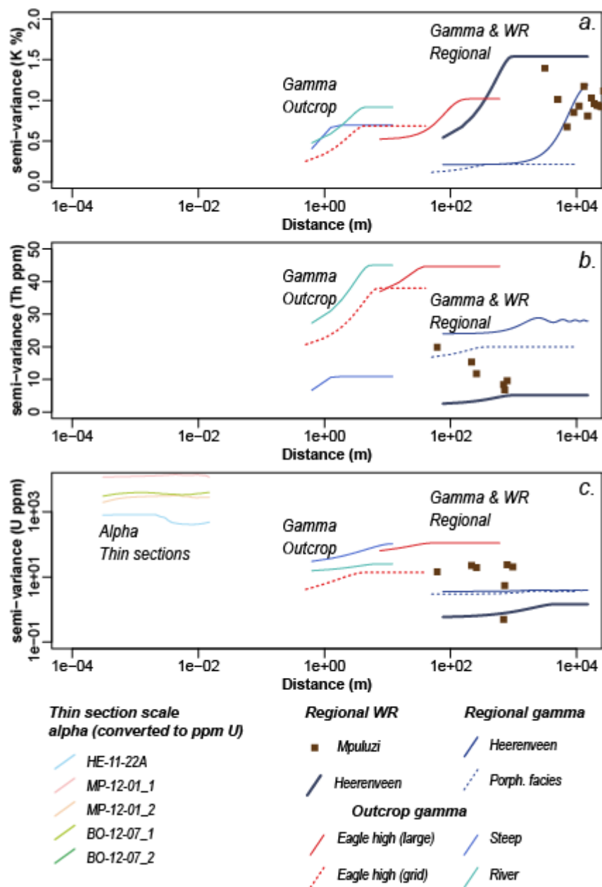
Figure 16. Compilation of the (model) variograms for the studied datasets for K (a), Th (b) and U (c). Each individual variogram (see EA6) is, for clarity, drawn using only the best fit model (lines), except for the Mpuluzi WR dataset where the variogram is too chaotic to fit a model.
