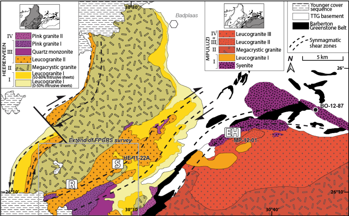
190 Figure 2. Geological map of the Heerenveen Batholith and adjoining portions of the Mpuluzi Batholith (Modified from Moyen et al., in press). Heerenveen after Belcher and Kisters (2006a ; b); Mpuluzi after Westraat et al. (2005). EH : Eagle High locality (Figure 10). R : « River » locality (Figure 8). S : « Steep » locality (Figure 9). The extent of the gamma-ray survey (corresponding to Figure 7) is also indicated, as well as the location of BeaQuant sample BO-12-87 of the Boesmanskop syenite (black circle, in the eastern part of the figure).
