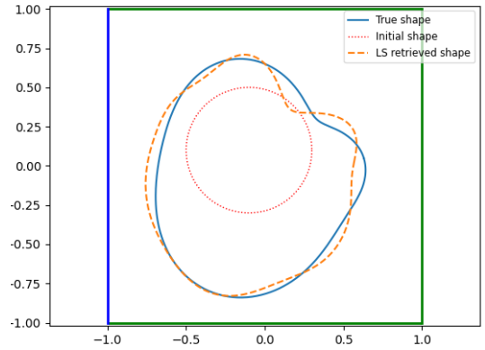
(a) Approximated object with least squares based shape inversion
