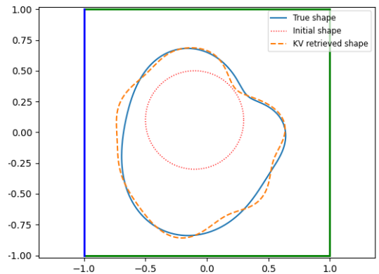
(b) Retrieved object with Kohn-Vogelius based shape inversion
