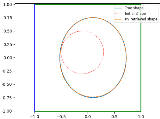
(b) Real and retrieved objects with the Kohn-Vogelius functional
