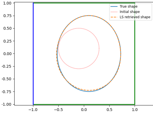
(a) Real and retrieved objects with the least squares cost functional
