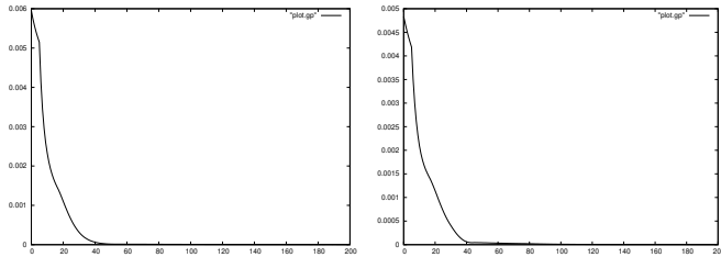
(a) Least squares functional convergence (b) Kohn-Vogelius functional convergence
