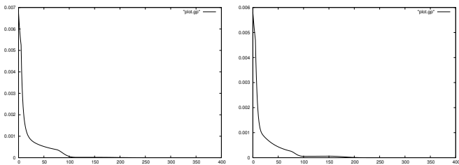
(a) Least squares cost functional convergence (b) Kohn-Vogelius cost functional convergence
