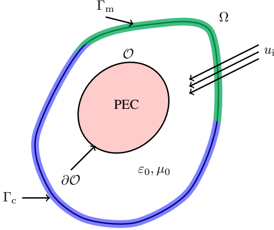
Fig. 1. Example of the considered domain \Omega with the scatterer \mathcal{O} (in red) inside.
