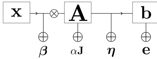
Figure 7. Additional nuisance sources. \mathbf{e} : additive white Gaussian noise of variance \sigma^2 . \eta , \beta : unwanted signal adding to the object signal. \alpha : constant offset added to the multiplexing matrix, \mathbf{J} : the matrix of ones. \eta , \beta and \alpha are real positive quantities and assumed to be known from a calibration step.
