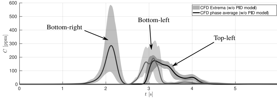
Figure 10: Variations between repetitions and phase-average of CFD-predicted concentration signals at the open surface
