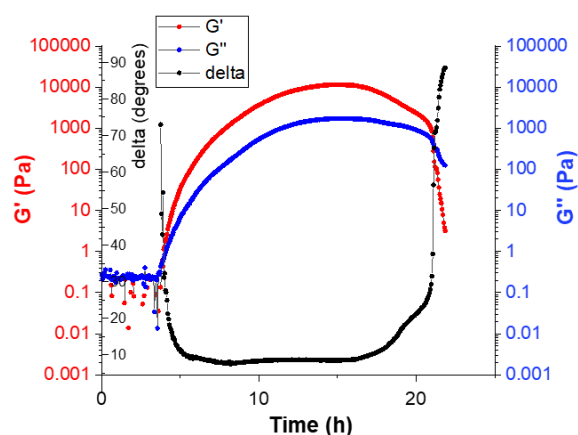
Figure 1: Elastic ( G' , red), viscous ( G'' , blue) modulus and dephasing (delta, black) of [\text{Zn}(\text{Cy})_2]/\text{octylamine} (OA) mixture over time. The monitoring is started 4 hours after mixing ( T = 0 h on the rheogram).
