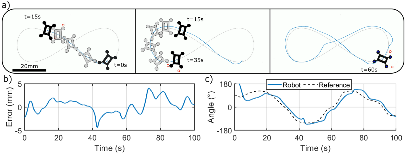
Fig. 7. Multiple-legged structure experimental path-following where the target orientation is perpendicular to the path. The control algorithm consists in (15) and (17) with K_{P_t} = K_{P_r} = 0.25 \text{ s}^{-1} , K_{I_t} = K_{I_r} = 0.025 \text{ s}^{-2} . a) The trajectory of the structure. Distance to the path (b) and orientation (c) error evolution. See supplementary video.
