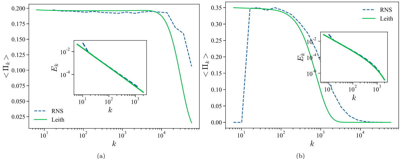
FIG. 7: Quantitative comparison of the energy transfers between RNS (dashed lines) and Leith-like transfers (full lines). The main figures present the two energy transfers, while the insets show the fitted energy spectra. The two figures are obtained for different values of \mathcal{R}_r (7a) \mathcal{R}_r \approx 2.23 (7b) \mathcal{R}_r \approx 3.34 .
