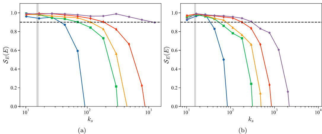
FIG. 15: Score \mathcal{S}(E) of the energy in each shell for \mathcal{G} = E . (15a) N = 12^3 ; (15b) N = 16^3 . Blue dots, green squares, orange triangles, red diamonds, and purple pentagons correspond to \nu = 10^{-4}, \nu = 10^{-5}, 5 \cdot 10^{-6}, 10^{-6}, 10^{-7} , respectively. Note that in (15a), the purple pentagons are associated with a quasi-thermalized state, being a crossover region between the two conjectures. Black dashed lines correspond to a score of 0.9.
