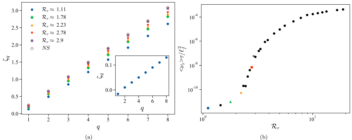
FIG. 5: Extracted exponents of the structure functions and localization in the transition for \lambda = \phi , N = 20^3 Modes. Both figures share the same legend. (5a) Exponents of the structure function of order q for various RNS simulations and comparison to a NS simulation. The inset presents the exponents, extracted at small scales, in the case of a quasi-thermalized state. (5b) Color coded version of the \nu_r vs \mathcal{R}_r diagram, showing where the various results are located with respect to the transition. The color of the data points are the same as those from panel (a).
