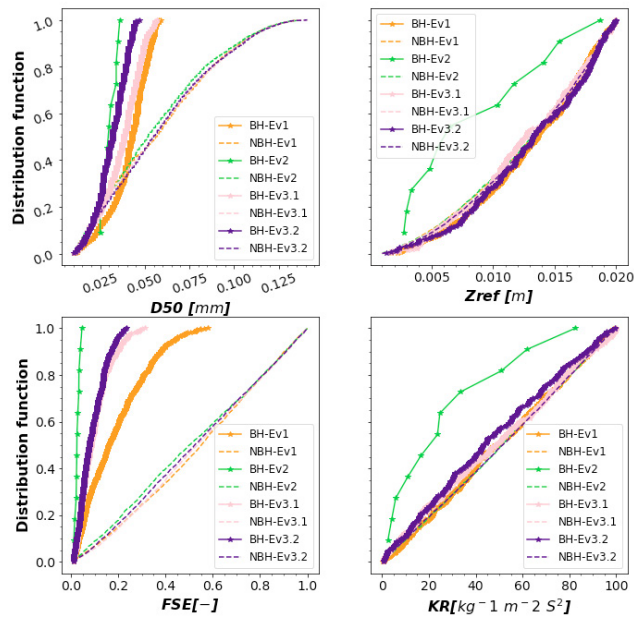
Figure 6. Posterior distributions for all the events and parameters: (top left) d_{50} , (top right) Z_{ref} , (bottom left) FSE , (bottom right) k_r (solid line: behavioral simulations, dashed line: non-behavioral simulations).
