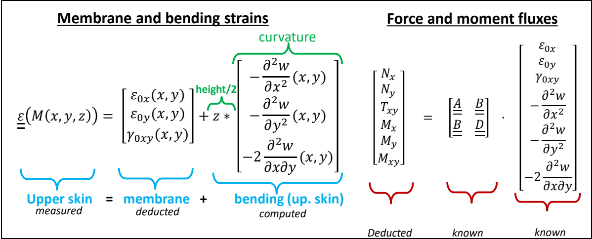
Figure 2: Obtaining the force and moment fluxes from the upper surface displacement using classical laminate theory [4]
