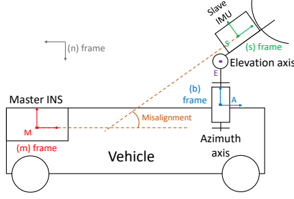
Fig. 1. Structure of the antenna positioning system
