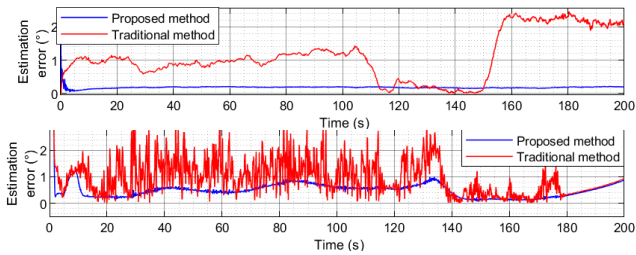
Fig. 3. Amplitude of the angle between estimated antenna direction and actual antenna direction, top: driving in relaxed off-road conditions, bottom: driving in intense off-road conditions
