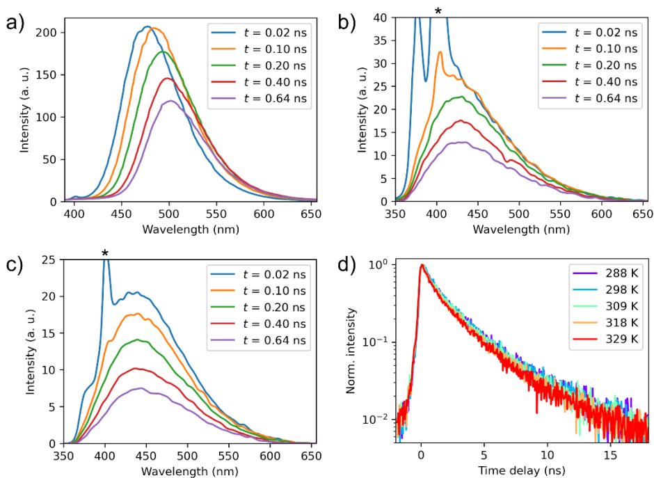
Figure 5. a) Photoluminescence emission of C481 in hexanol at different times ( t ) post-excitation ( \lambda_{\text{ex}} = 355 \text{ nm} ); b) Photoluminescence emission of PolyDHP in hexanol at different times ( t ) post-excitation ( \lambda_{\text{ex}} = 355 \text{ nm} ); c) photoluminescence emission of PolyDHP in THF at different times ( t ) post-excitation at room temperature ( \lambda_{\text{ex}} = 355 \text{ nm} ); d) Photoluminescence decays of PolyDHP at varying temperature in the range 278 – 330 K in THF ( \lambda_{\text{ex}} = 355 \text{ nm} ) measured in spectral region 425 – 475 nm. Asterisks indicate Raman scattering signals.
