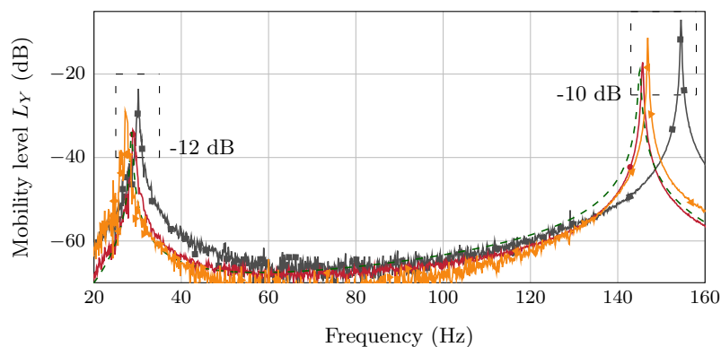
Figure 12: Plate mobility in dB with: (—●—) measured MPP⑦ shown in Figure 11, (—■—) measured reference non-perforated plate ②, (—▲—) measured reference MPP with d = d_1 and (---) theoretical MPP⑦. MPP⑦ is considered as three equivalent MPP inhomogeneous spatial distribution of perforations defined in Equation (29). Spatial distribution (29a) associated with d_1 = 1.3 \text{ mm} while spatial distributions (29b) and (29c) are related to d_2 = 0.7 \text{ mm} . Loss factor and Young's modulus used in the theoretical model are obtained experimentally from measurements on the non-perforated plate.
