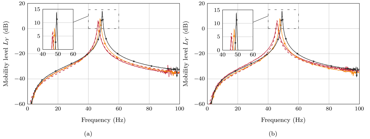
Figure 10: Theoretical and experimental mobilities around mode 1 of (a) MPP⑤ and (b) MPP⑥. Comparisons between (—) measured and (---) theoretical. In (a) and (b), the measured mobilities of the reference MPP④ (—▲) and non-perforated plate (—■) are also provided. MPP perforation parameters are given in Figure 9(b).
