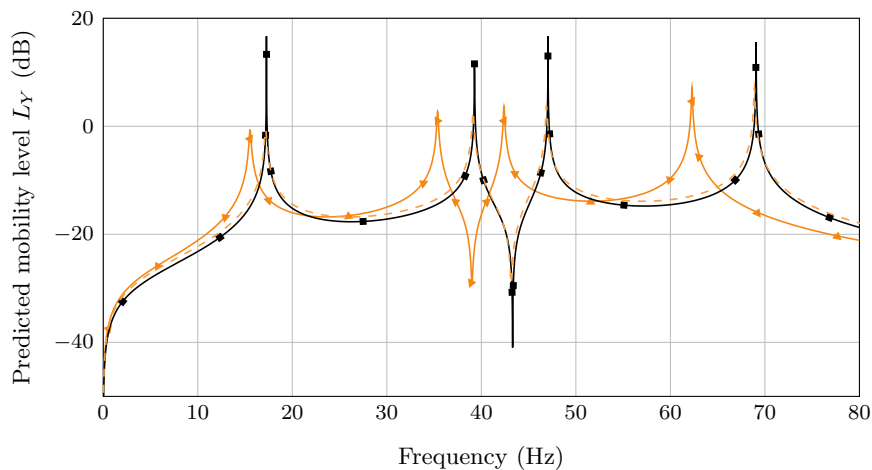
Figure 2: Predicted mobility level of aluminum plates of dimensions 490 \text{ mm} \times 570 \text{ mm} \times 1 \text{ mm} : (—■) reference non-perforated plate, (—▲) MPP with a perforation diameter, denoted d_1 , set to induce maximum added damping in the first MPP mode, and (---) MPP with the same equivalent stiffness as the reference non-perforated plate and with d \equiv d_1 maximizing the added damping on the first MPP mode. Perforation parameters are d_1 = 1.6 \text{ mm} and \phi^{(0)} = 10\% . Isotropic structural loss factor of aluminum \eta_s = 10^{-4} or 0.01% is also considered.
