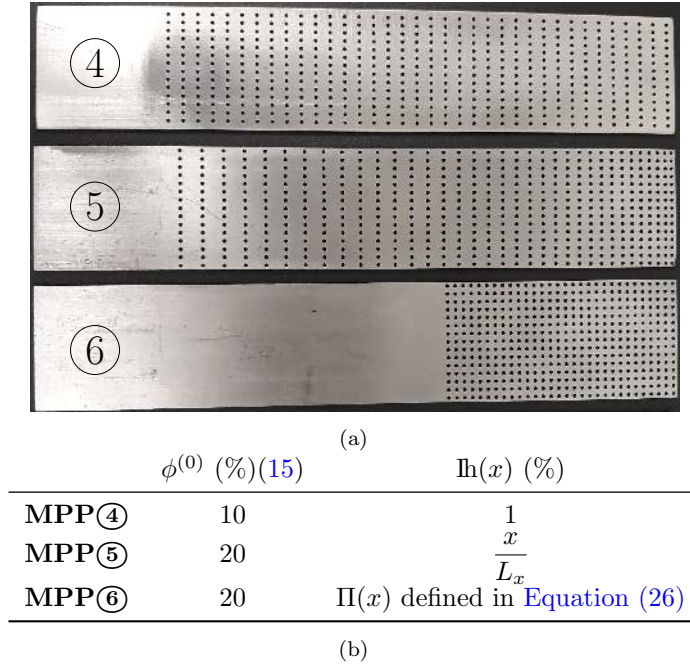
Figure 9: Tested MPP samples with various space-dependent distributions of the perforation ratio. (a) — MPP④ homogeneous distribution: reference MPP, MPP⑤ linear distribution, MPP⑥ concentrated distribution located at the maximum of the deflection amplitude. (b) — Perforation parameters and homogeneity function \text{Ih}(x) for the three MPP presented in Figure 9(a). Perforation diameter is set to d = 1 mm in order to induce maximum damping around the first mode (i.e. i = 1 ) and global perforation ratio \phi_g = 10\% identical for all three MPP.
