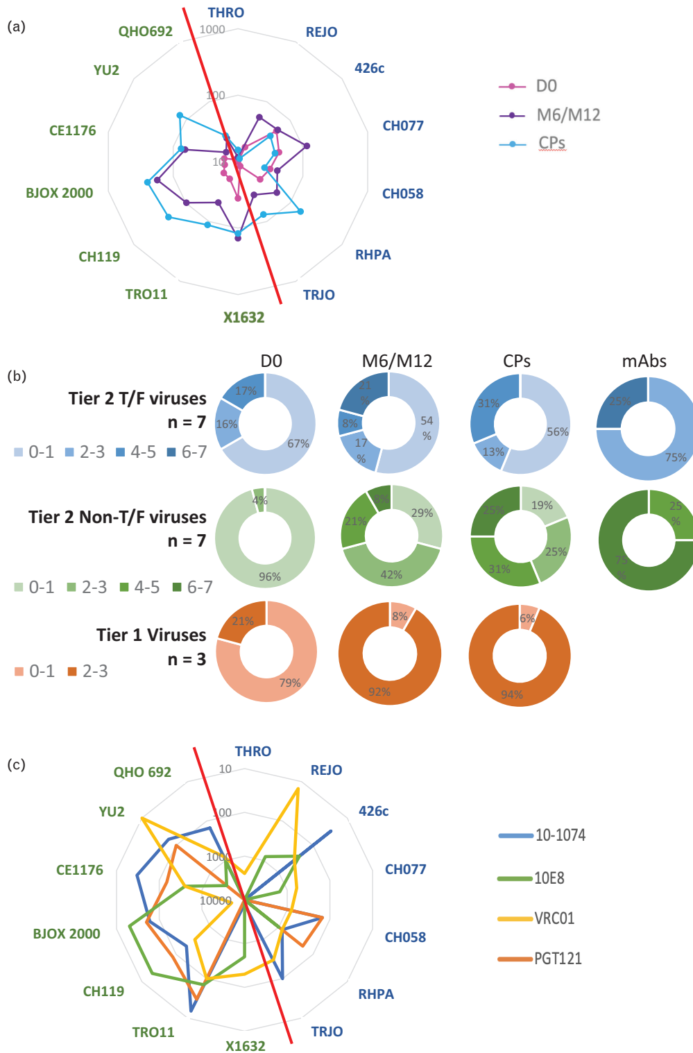
Fig. 2. Detection of cross-neutralizing activity against transmitted founder (T/F) viruses at D0. Radar chart against T/F viruses (in blue) and non-T/F (in green) for mean inhibitory reciprocal dilution 50% (IRD50) neutralizing activities of sera collected at three time points (a) or inhibitory concentration 50 (IC50) of four bnNAb: 10-1074 and PGT121 targeting V3 glycan-dependent epitopes, 10E8 targeting the remarkably conserved gp41 membrane-proximal external region and VRC01 targeting the conformational CD4 + -binding site. (c). Pie charts representing the percentage of viruses neutralized with an IRD50 value of at least 50 for sera collected at D0, M6/M12 and chronic progressors or IC50 less than 1 \mu\text{g/ml} for bnNAb 10-1074, PGT121, 10E8 and VRC01 for Tier 2 T/F (blue), non-T/F (green) and Tier 1 (orange) strains (b).
