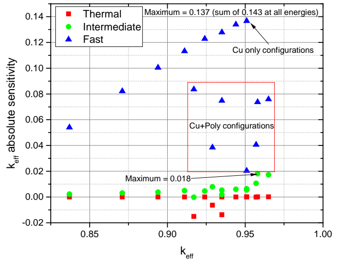
Fig. 6. k_{eff} sensitivity to Cu-63 as a function of k_{eff} .
