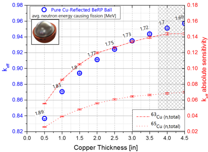
Fig. 5. MCNP ® results for all Cu-reflected BeRP Ball base configurations highlighting the simulated k_{eff} , average neutron energy causing fission, and absolute copper total cross section sensitivity.
