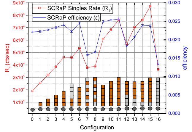
Fig. 11. Count rate ( R_1 ) and detector efficiency ( \varepsilon ) for SCRaP configurations.
