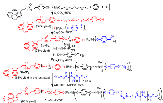
Scheme 14. Synthesis of a pyrene derivative equipped with a long chain, and its use as core of dendrons, up to dendron 3b-G'1-PVDF , functionalized with 10 poly(vinylidene fluoride) chains on its surface.
