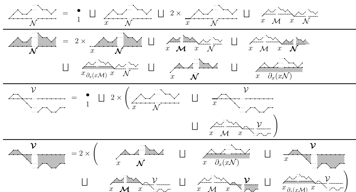
Figure 5: The decompositions of lattice paths in \mathcal{N} , \mathcal{N} , \mathcal{V} , and \mathcal{V} from Theorem 20, Theorem 21, Theorem 22, and Theorem 23.
