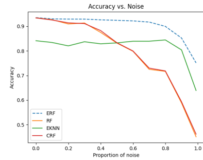
(f) Ionosphere
