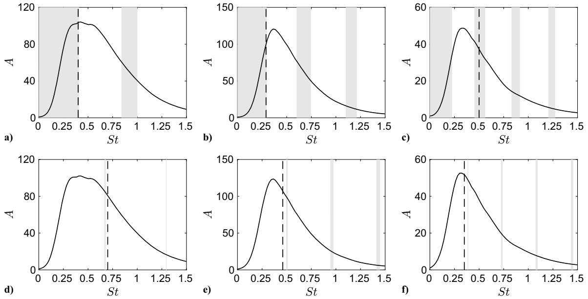
Fig. 21 Power gain of the Kelvin–Helmholtz waves between z = 0 and 8r_0 as a function of the Strouhal number for (top) n_\theta = 0 and (bottom) n_\theta = 1 for (a, d) M = 0.9 , (b, e) M = 1.1 , and (c, f) M = 1.3 : - - - dominant near-nozzle tone frequency; (light-gray shading) allowable frequency bands of the free-stream upstream-propagating guided jet waves.
