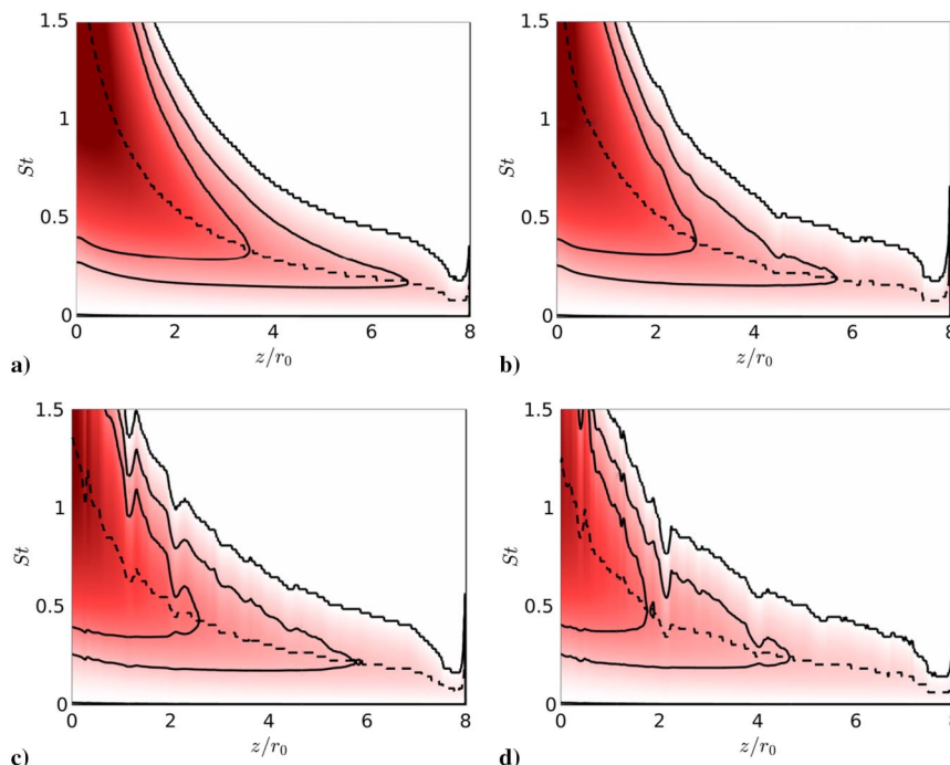
Fig. 20 Instability growth rates -k_i r_0 for n_\theta = 0 as a function of the axial position z and of the Strouhal number St at a) M = 0.6 , b) M = 0.9 , c) M = 1.1 and d) M = 1.3 , - - most unstable frequencies. Contour lines for the levels 0, 0.5 and 1 are drawn in black. The color scale ranges from 0 to 3, from white to red.
