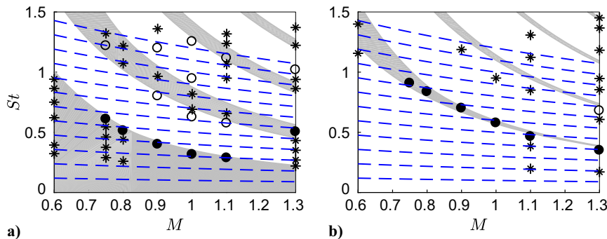
Fig. 8 Mach number variations of the Strouhal numbers of the peaks in the near-nozzle pressure spectra for a) n_\theta = 0 and b) n_\theta = 1 : \bullet and \circ dominant tones and their harmonics; * other peaks; (gray shading) allowable frequency bands of the free-stream upstream-propagating guided jet waves for a vortex-sheet model; - - Eq. (1) with N varying from 1 to 12.
