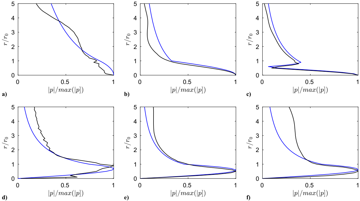
Fig. 18 — Radial profiles of rms pressure for the components with k < 0 from the LES and — pressure eigenfunctions of the upstream-propagating free-stream guided jet waves given by a vortex-sheet model [16] for (top) n_\theta = 0 and (bottom) n_\theta = 1 and (a, d) M = 0.6 , (b, e) M = 0.9 and (c, f) M = 1.3 .
