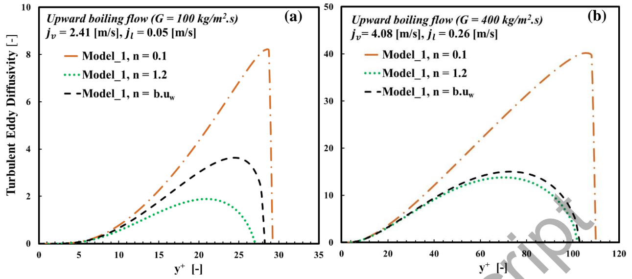
Figure 5. Eddy viscosity versus dimensionless distance from the wall in upward flow. (a) G = 100 \text{ kg/(m}^2\text{s)} , (b) G = 400 \text{ kg/(m}^2\text{s)} .
