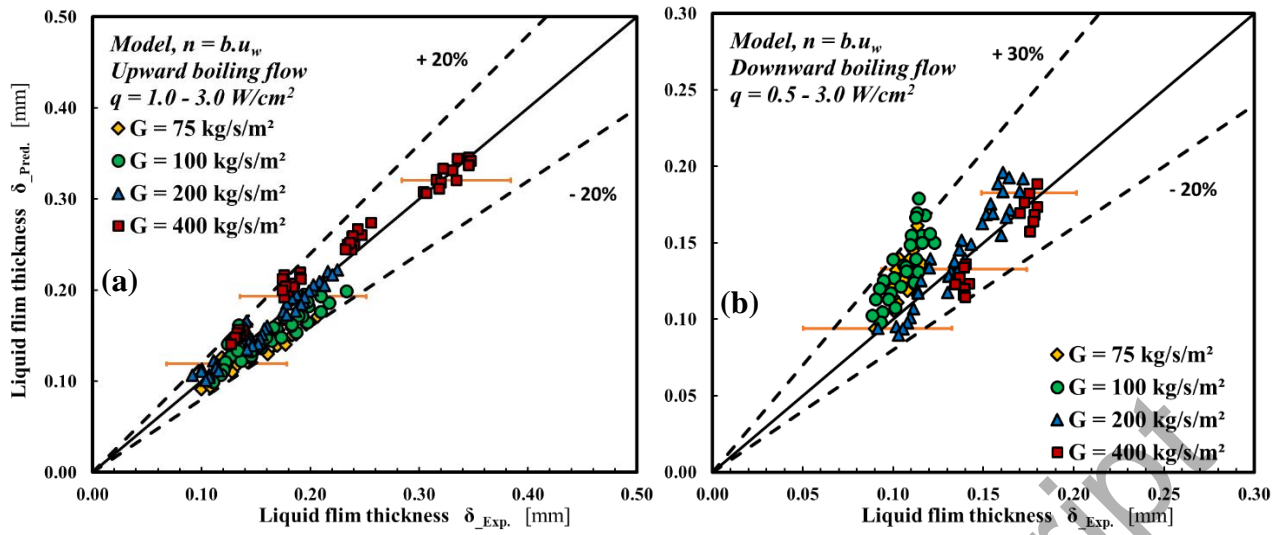
Figure 12. Predicted versus measured film thickness in the annular flow regime, (a) upward flow and (b) downward flow.
