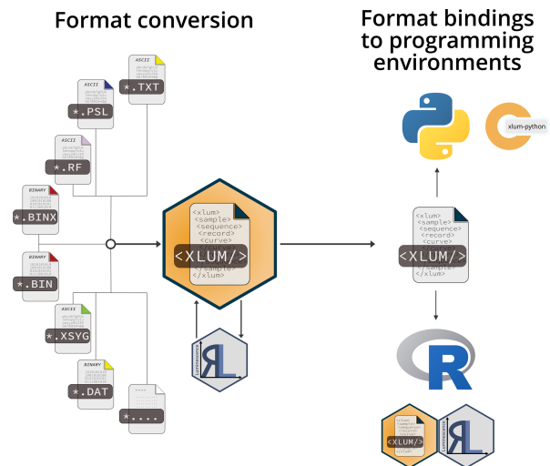
Figure 5. The R package xlum supports the conversion of various commonly used luminescence (dating) data formats to <xlum/> using the R package Luminescence . Bindings to the statistical programming language R and the general-purpose programming language Python are realised through language-specific software packages.
