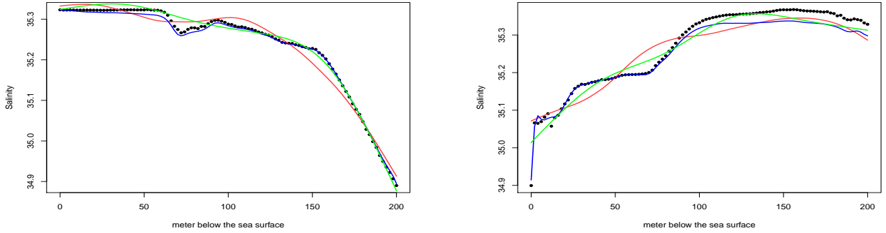
Figure 12: Prediction given by the three methods for integral model on two randomly chosen observations in the test sample: PenFFR in blue, PFFR in green and wSigcomp in red. Black dots are the true values.
