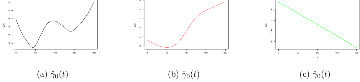
Figure 11: Estimates \hat{\gamma}_0(t) , 1 \leq j \leq 4 for the three methods: wSigcomp (left column), integral PFFR (middle column) and integral PenFFR (right column).
