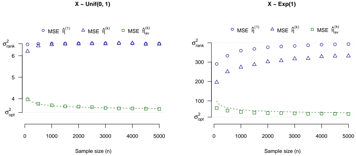
Figure 3: Evolution of the MSE's of the estimators \hat{\eta}^{(1)} , \hat{\eta}^{(k)} and the average \hat{\eta}_{av}^{(k)} with k = \lfloor n^{1/3} \rfloor , as a function of n in the model Y = \sin(5X) + 2X\epsilon , under uniform (left) and exponential (right) distribution of the inputs. The MSEs are multiplied by the sample size n to highlight the convergence as n \rightarrow \infty . The values are obtained from Monte-Carlo estimations with N = 10^5 repetitions. The green dashed line represents the MSE first order asymptotic expansion for the averaged estimator derived from Equation (3).
