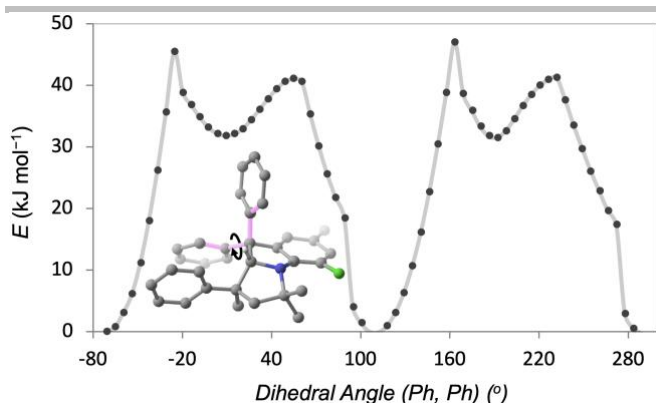
Figure 4. Gear behavior of (S,R)-2b upon clockwise rotation of the equatorial phenyl group ( r^2 SCAN-3c(SMD=CH 2 Cl 2 ). For other rotational modes, see Figs. S5–S9.
