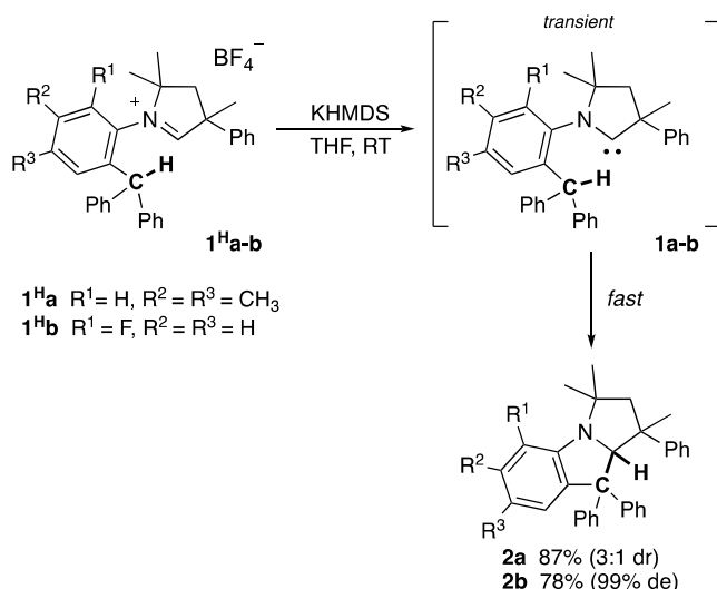
Scheme 1. Synthesis of racemic compounds 2a-b .
