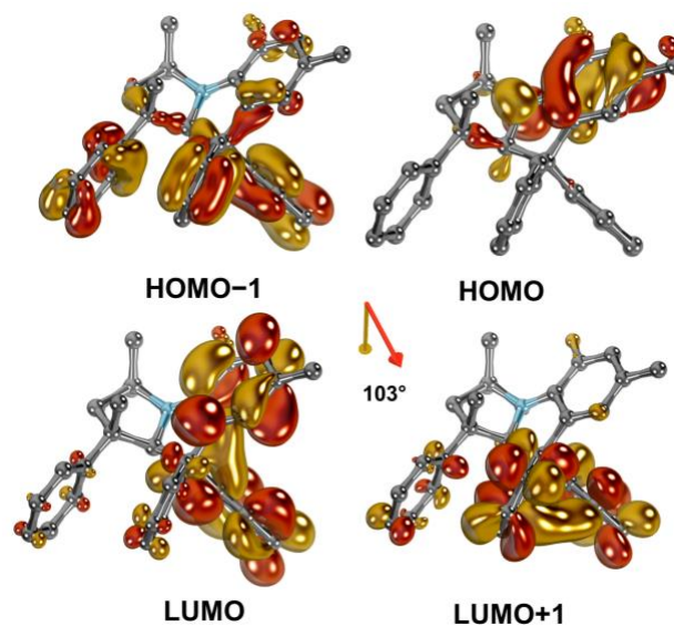
Figure 6. The HOMO-1, LUMO and LUMO+1 suggest chiral exciton coupling. The transition electric dipole moment vector for the transition to the S_1 excited state (HOMO→LUMO transition) is given in red, the transition magnetic dipole moment vector in gold, hydrogen atoms are omitted for clarity.
