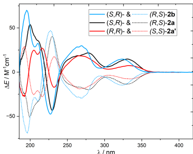
Figure 5. ECD spectra of (S,R)- and (R,S)-2b (solid and dotted blue lines, respectively), (S,R)- and (R,S)-2a (solid and dotted black lines, respectively) and (R,R)- and (S,S)-2a' (solid and dotted red lines, respectively) measured in acetonitrile ( \sim 10^{-5} \text{ M} ) at 298 K.
