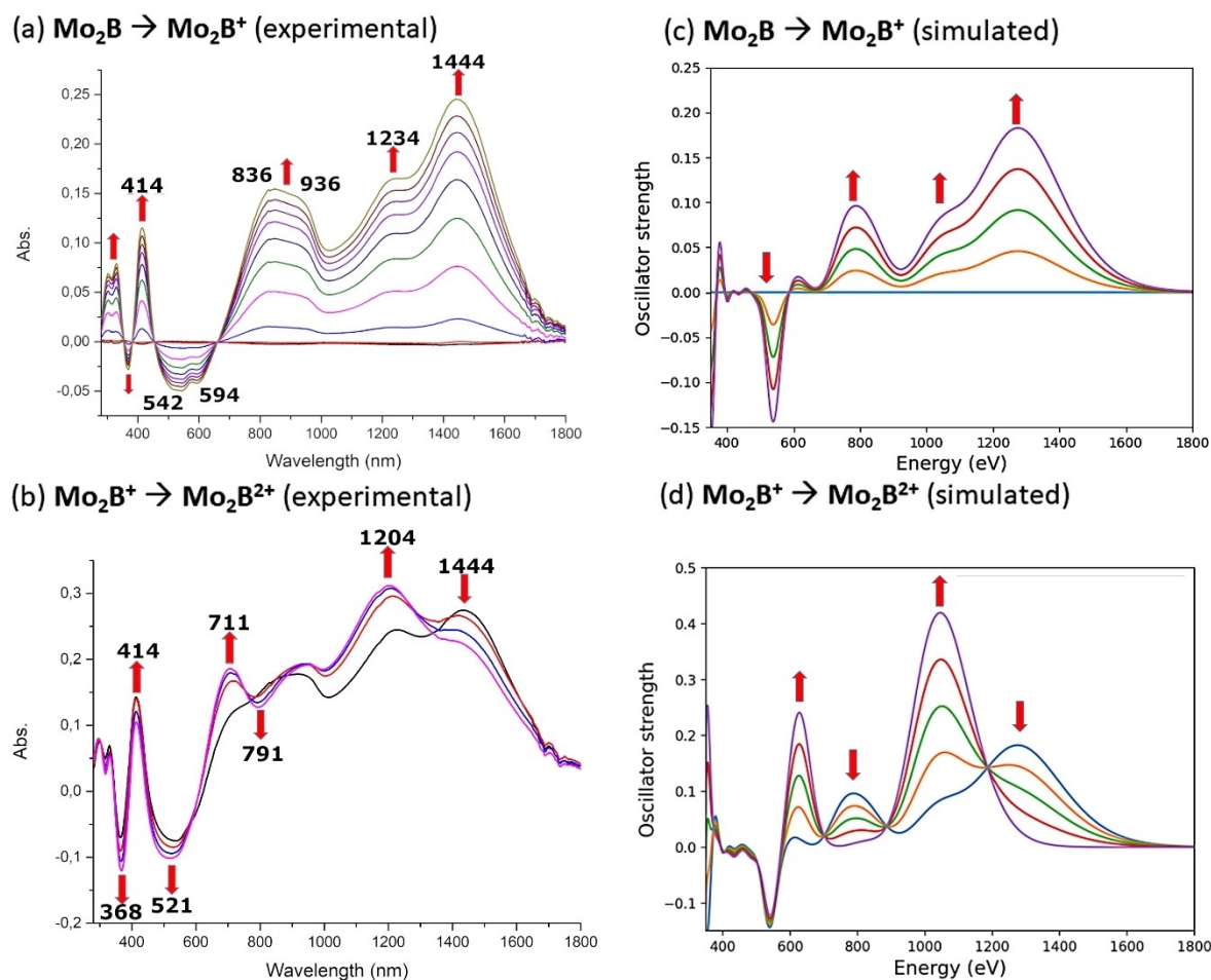
Figure 4. Experimental (a,b) and simulated (c,d) differential UV-vis-NIR absorption spectra of Mo 2 B , monitored from neutral to radical cation state (a,c), from radical cation to dication state (b,d).
